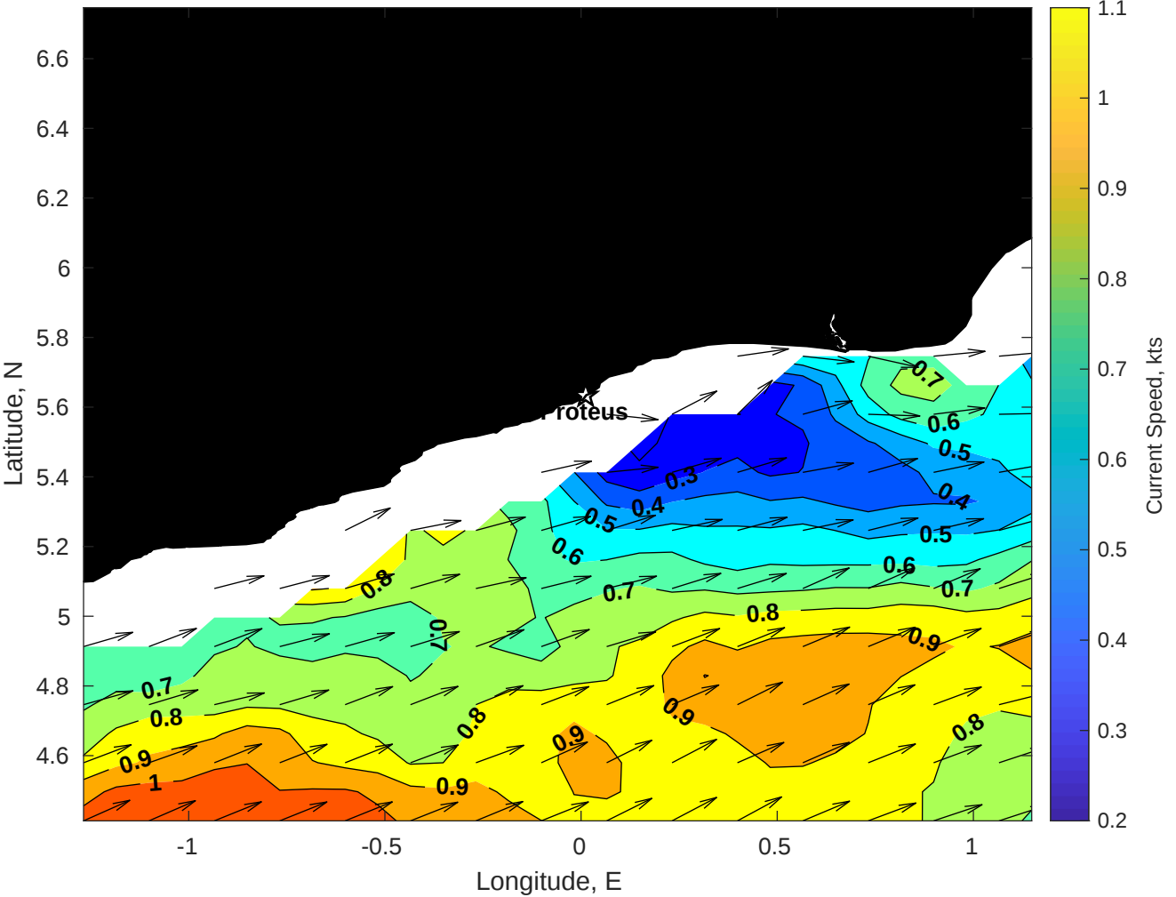
Surface Currents for Proteus at 14-Sep-2025 00:00:00
