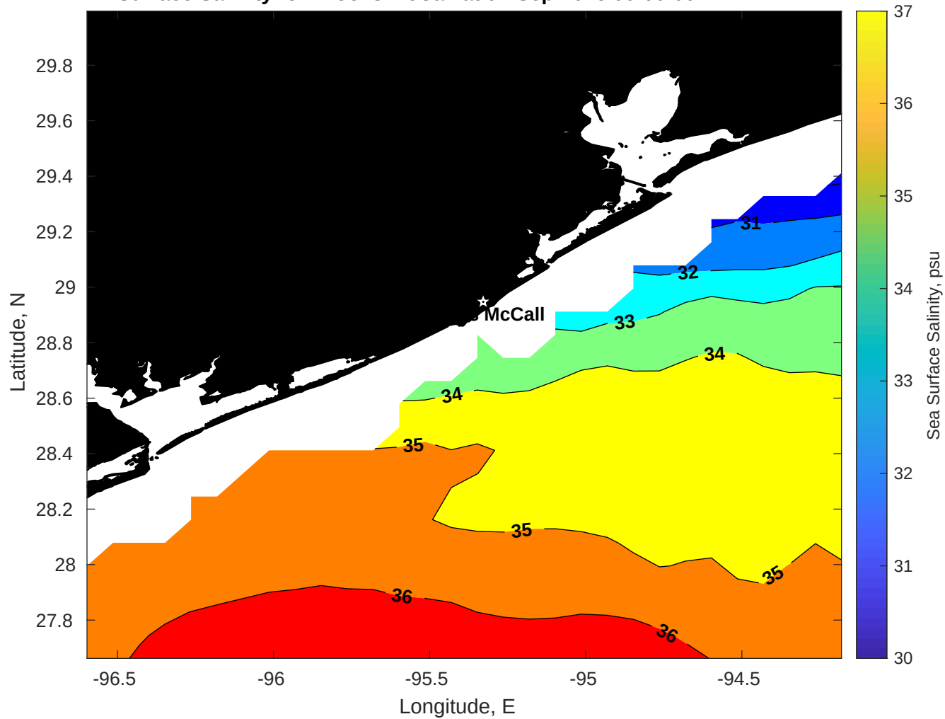
Surface Salinity for Brooks McCall at 01-Sep-2025 00:00:00
