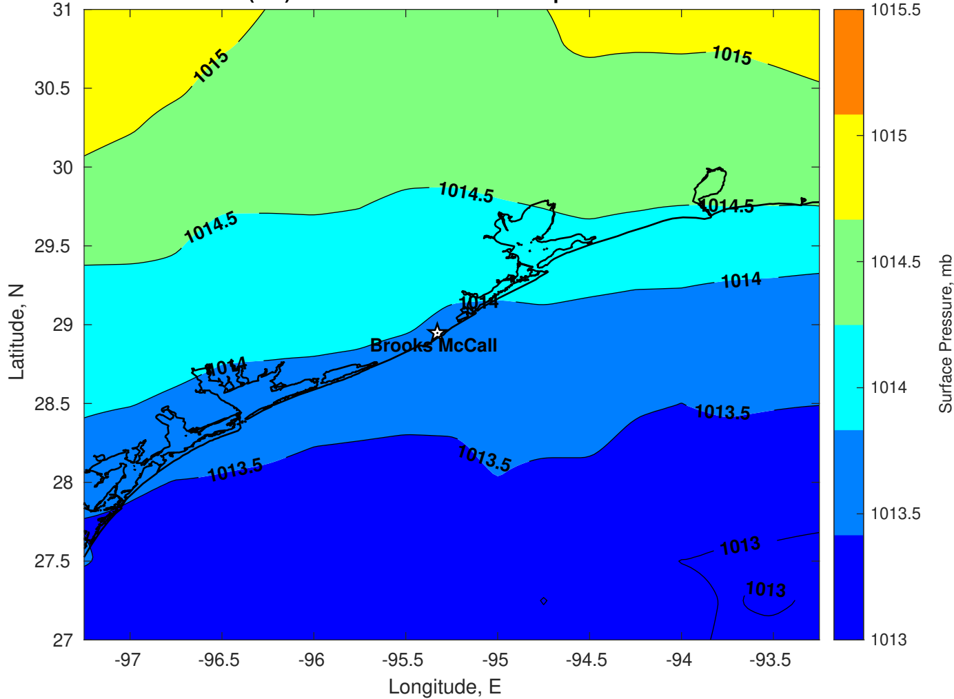
Surface Pressure (mb) for Brooks McCall at 02-Sep-2025 12:00:00
