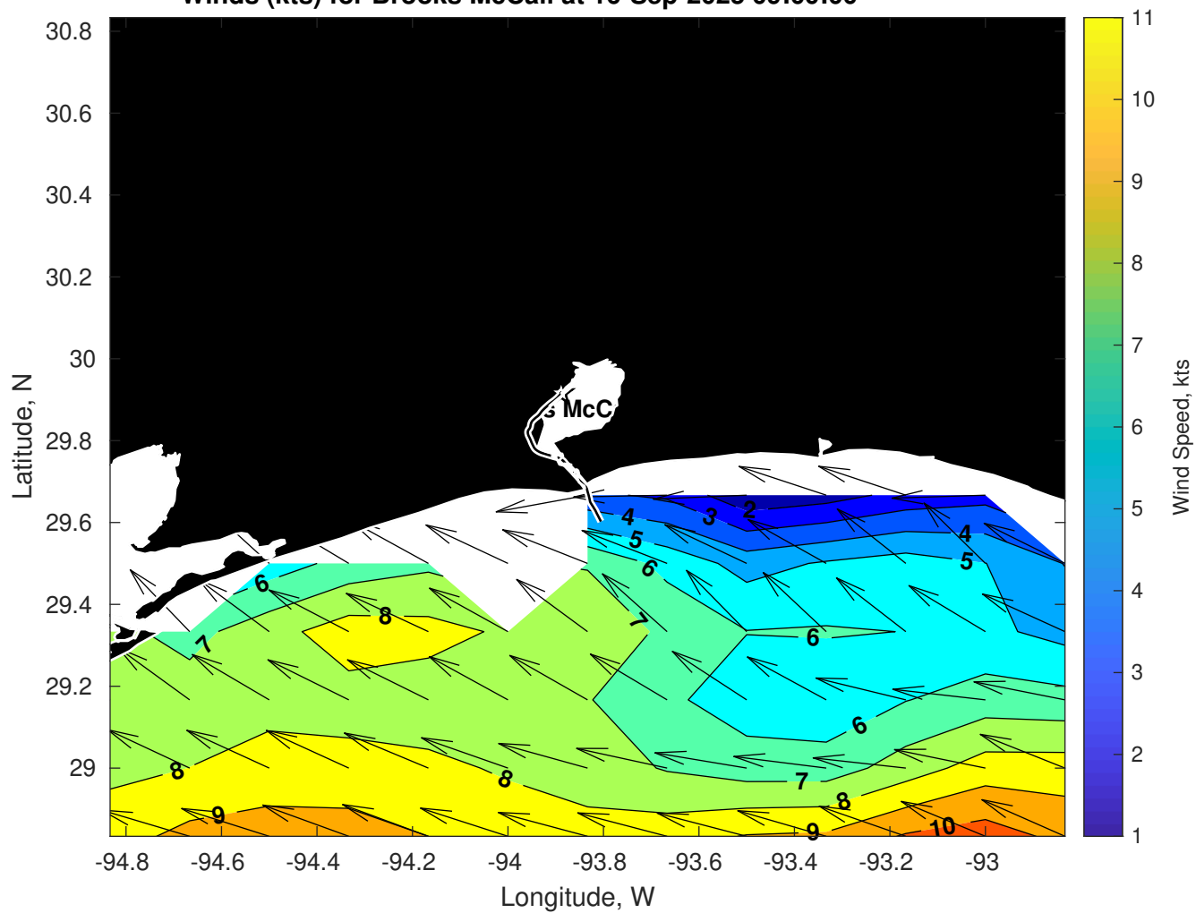
Winds (kts) for Brooks McCall at 16-Sep-2025 09:00:00
