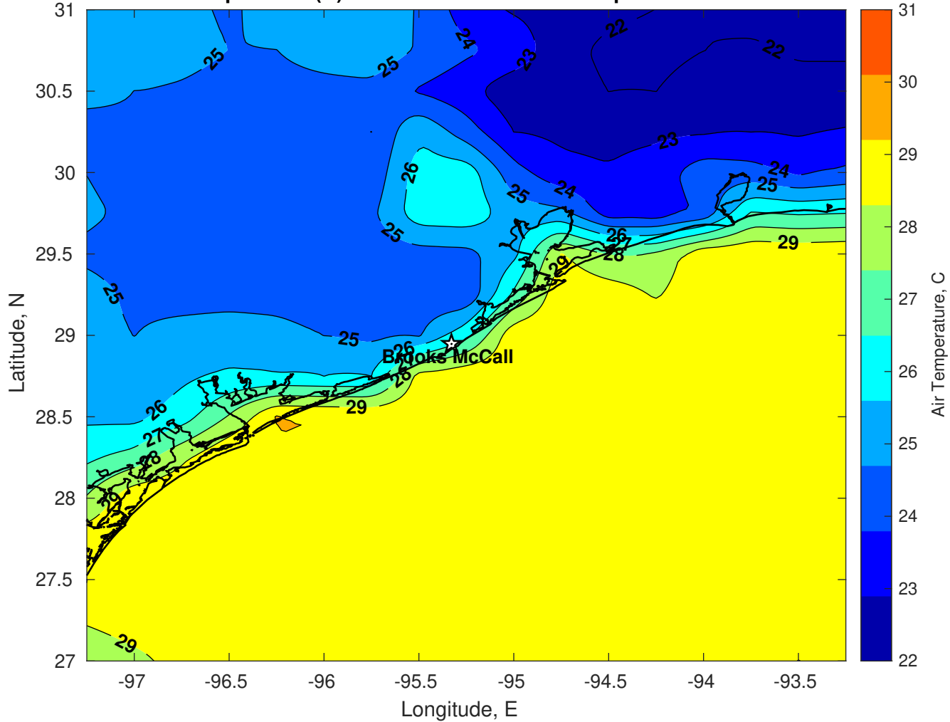
Air Temperature (C) for Brooks McCall at 16-Sep-2025
