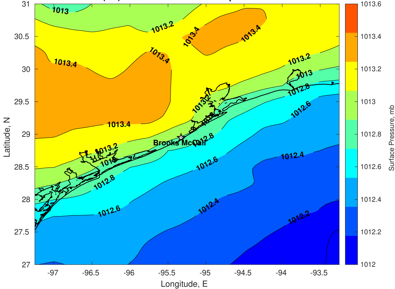
Surface Pressure (mb) for Brooks McCall at 03-Sep-2025 12:00:00
