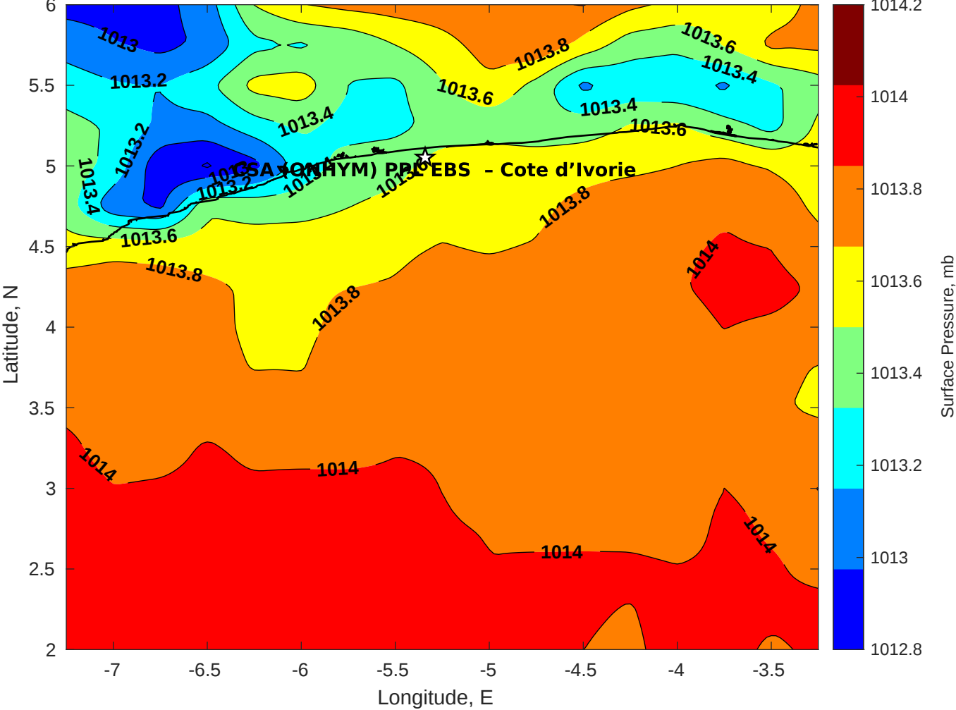
Surface Pressure (mb) for CSA (ONHYM) PPL EBS - Cote d'Ivoire at 16-Sep-2025 12:00:00
