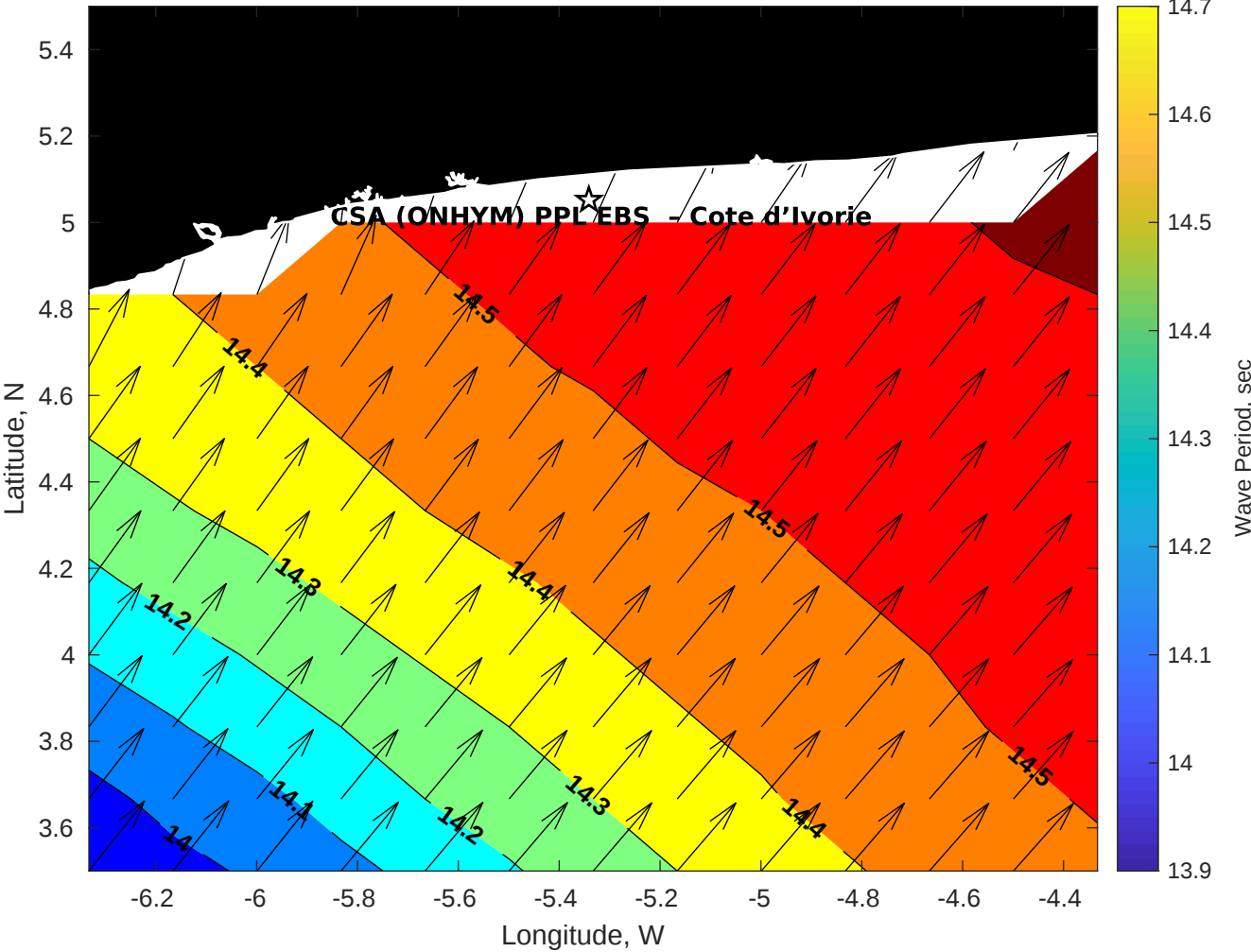
Wave Period (sec) for CSA (ONHYM) PPL EBS - Cote d'Ivoire at 16-Sep-2025 09:00:00
