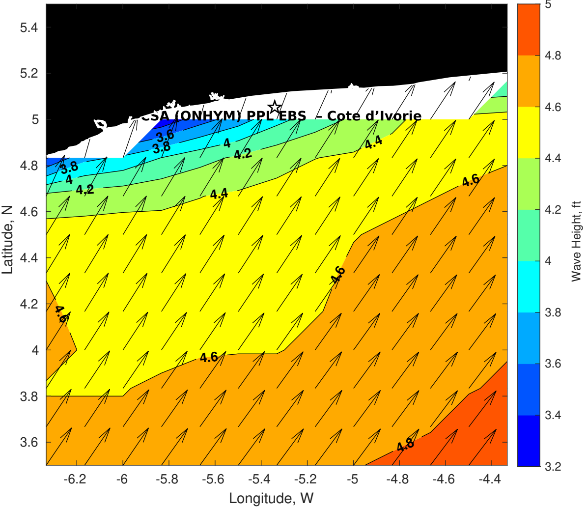
Wave Height (ft) for CSA (ONHYM) PPL EBS - Cote d'Ivoire at 16-Sep-2025 09:00:00
