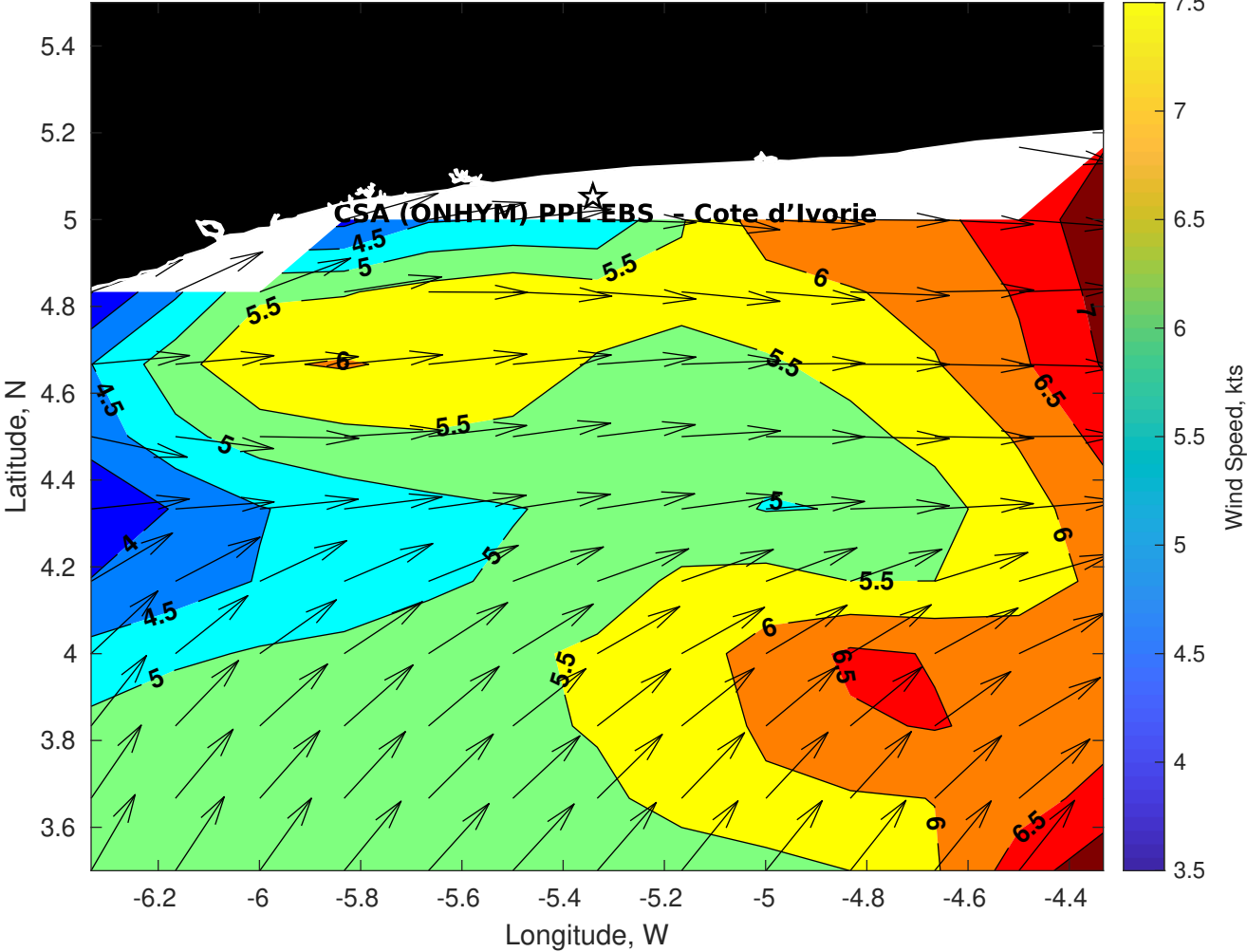
Winds (kts) for CSA (ONHYM) PPL EBS - Cote d'Ivoire at 16-Sep-2025 09:00:00
