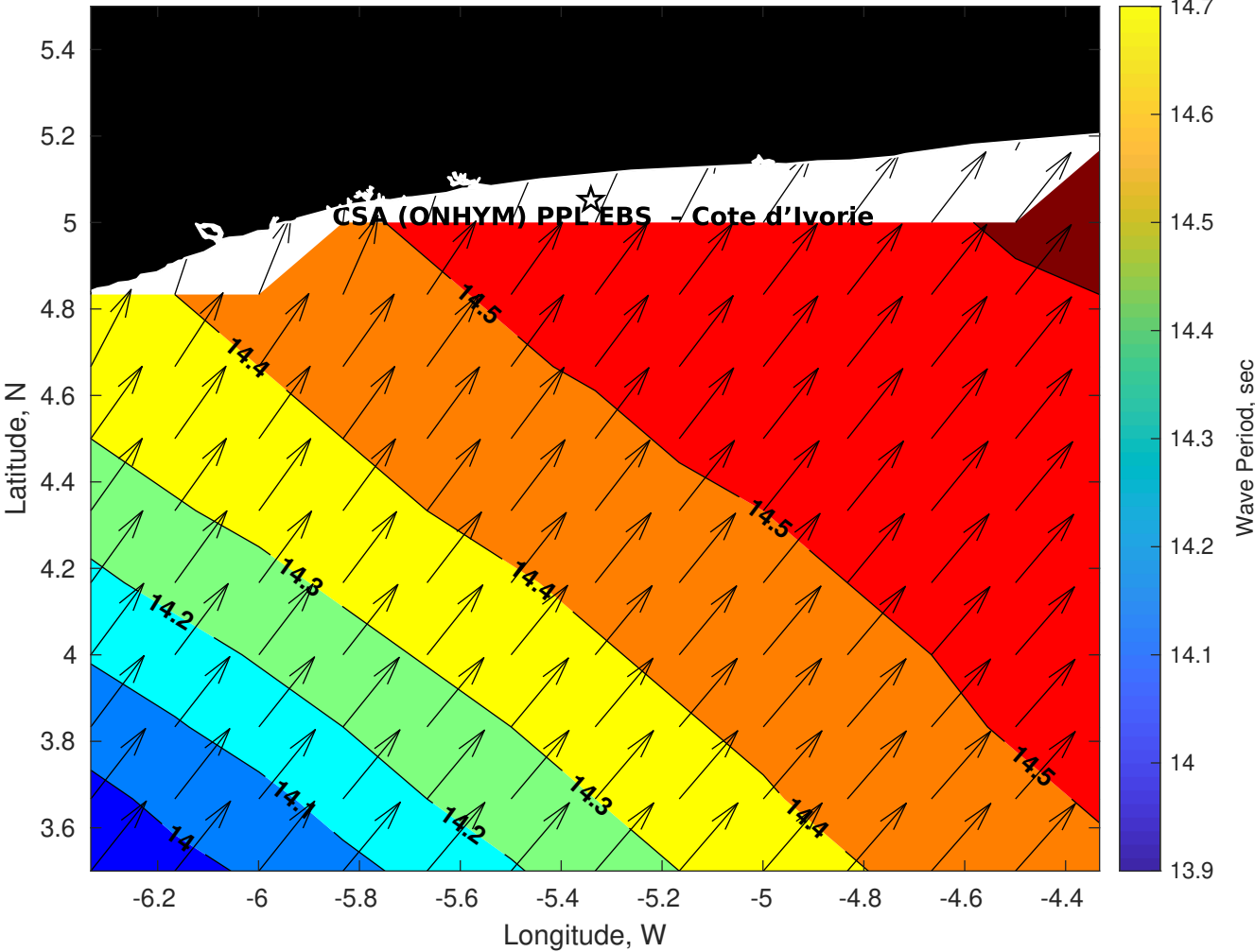
Wave Period (sec) for CSA (ONHYM) PPL EBS - Cote d'Ivoire at 16-Sep-2025 09:00:00
