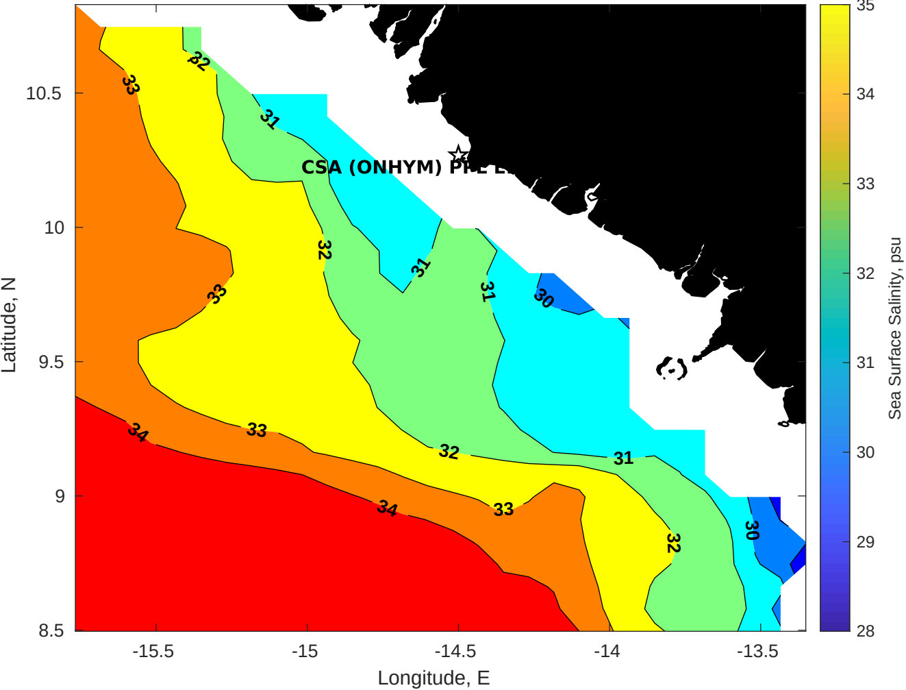
Surface Salinity for CSA (ONHYM) PPL EBS - Guinea at 15-Sep-2025 00:00:00
