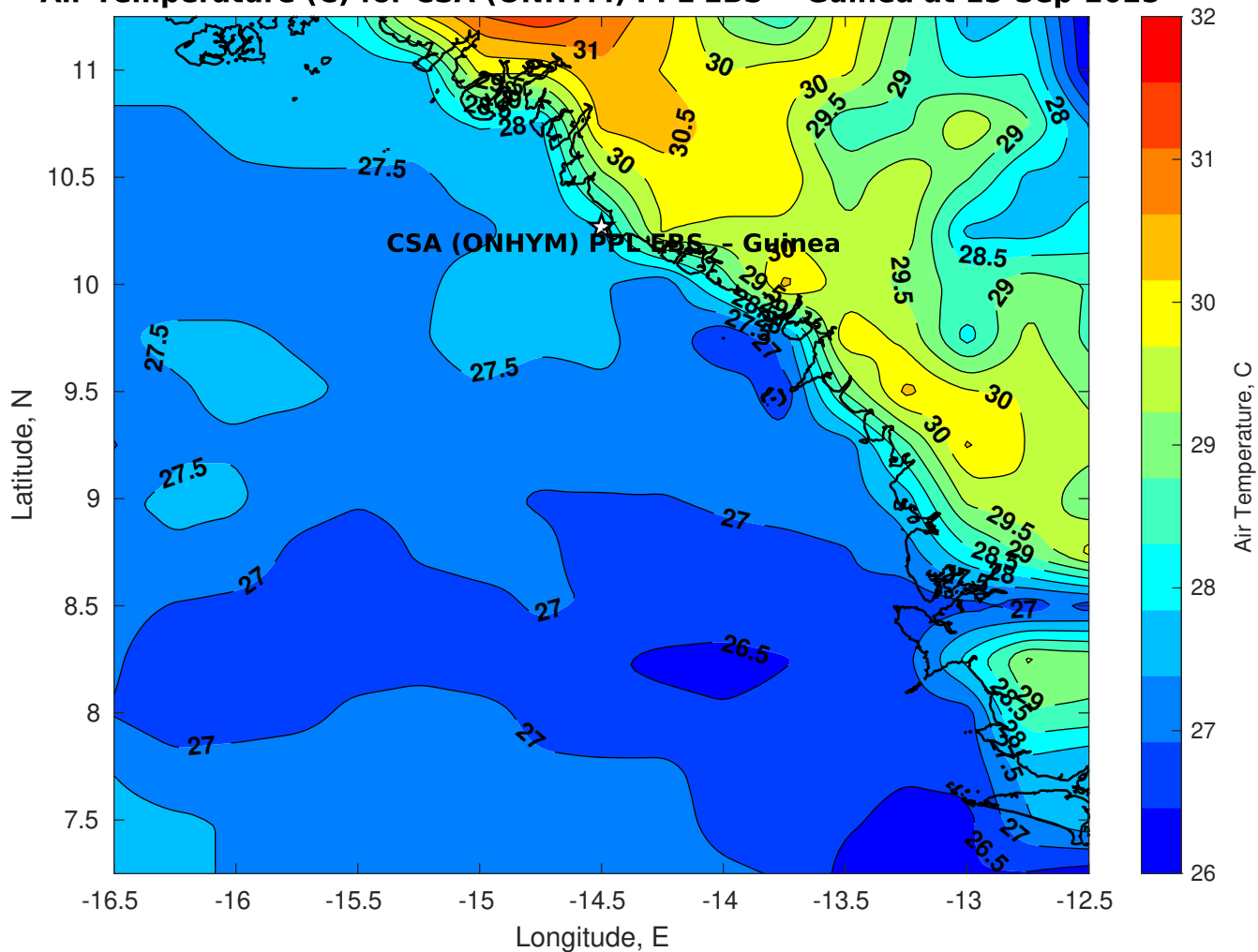
Air Temperature (C) for CSA (ONHYM) PPL EBS - Guinea at 15-Sep-2025
