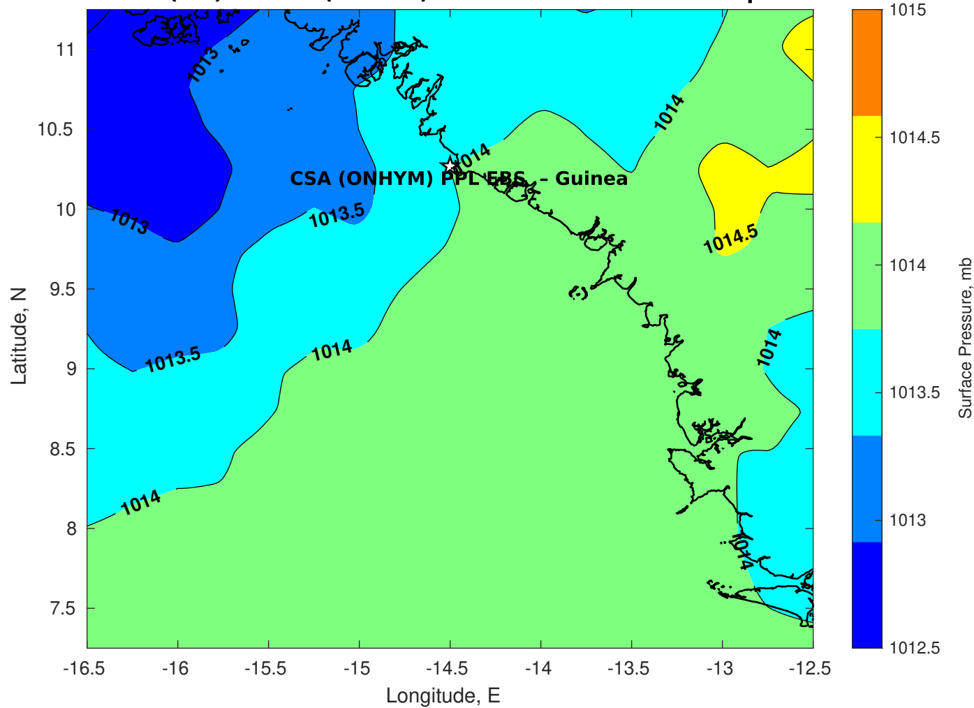
Surface Pressure (mb) for CSA (ONHYM) PPL EBS - Guinea at 16-Sep-2025 12:00:00
