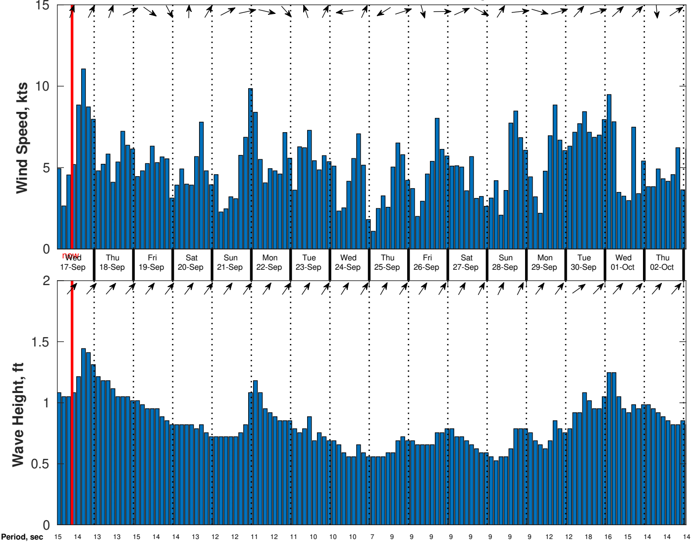
Wind & Wave Forecast for CSA (ONHYM) PPL EBS - Guinea from 16-Sep-2025 01:00:00 to 02-Oct-2025 01:00:00
