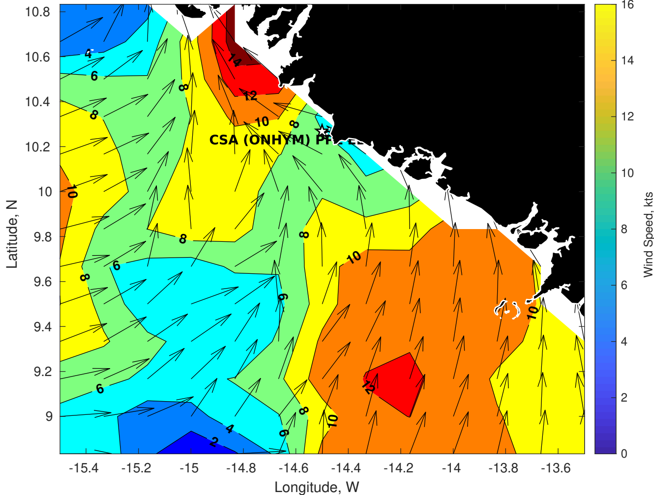
Winds (kts) for CSA (ONHYM) PPL EBS - Guinea at 16-Sep-2025 09:00:00
