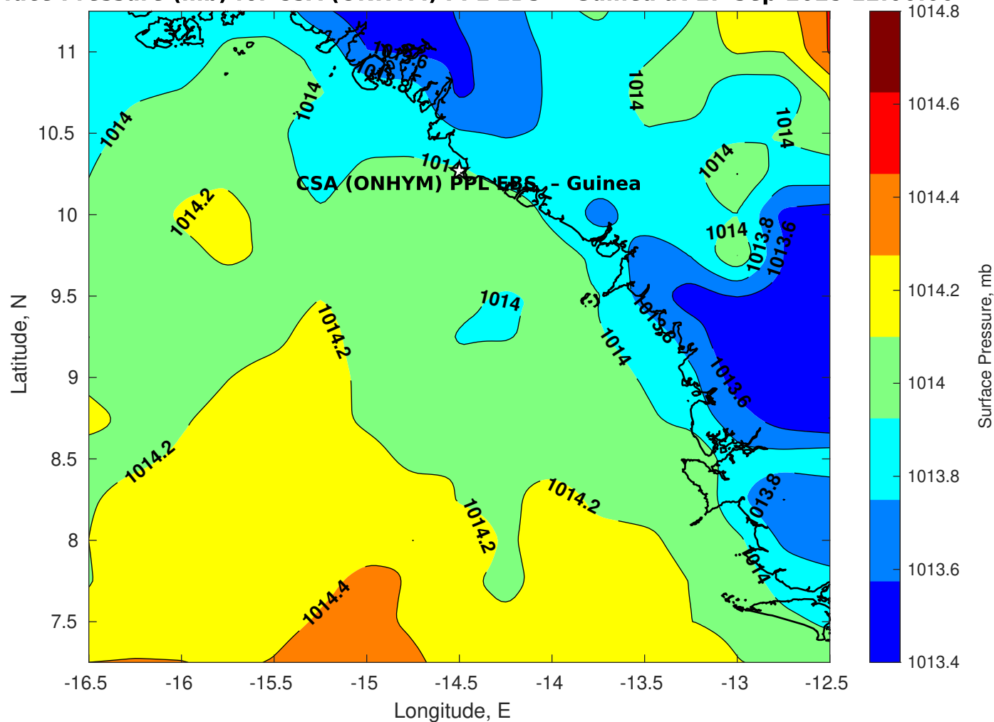
Surface Pressure (mb) for CSA (ONHYM) PPL EBS - Guinea at 17-Sep-2025 12:00:00
