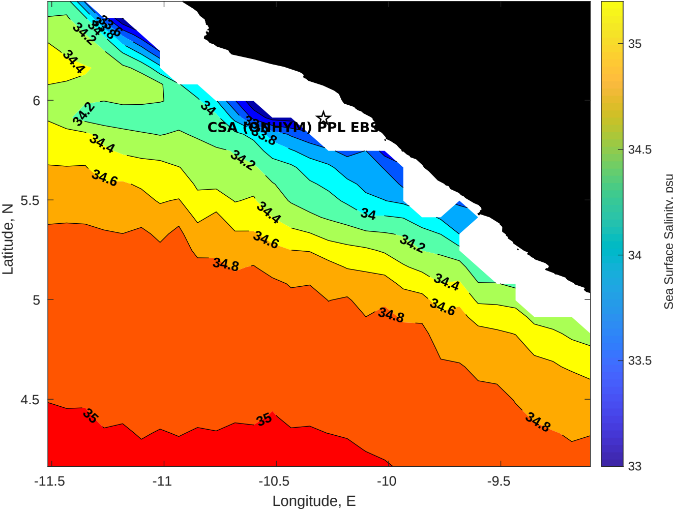
Surface Salinity for CSA (ONHYM) PPL EBS - Liberia at 15-Sep-2025 00:00:00
