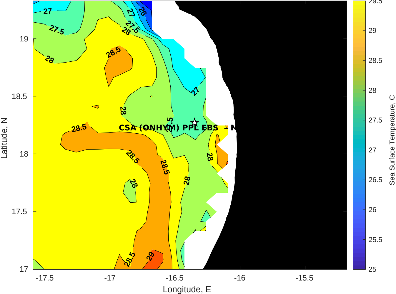
SST for CSA (ONHYM) PPL EBS - Mauritania at 15-Sep-2025 00:00:00
