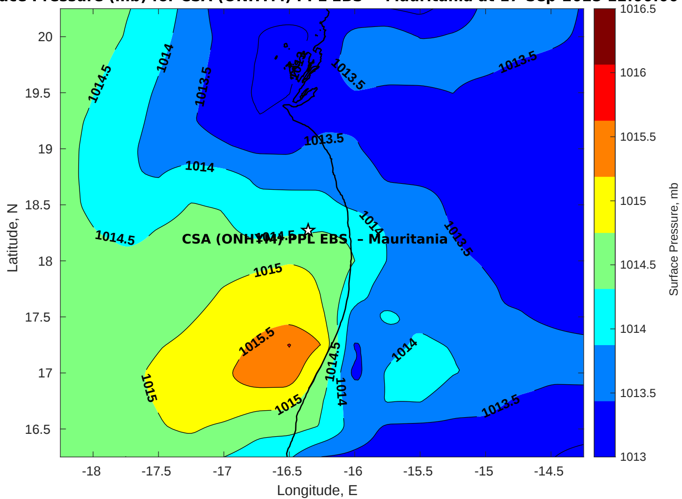
Surface Pressure (mb) for CSA (ONHYM) PPL EBS - Mauritania at 17-Sep-2025 12:00:00
