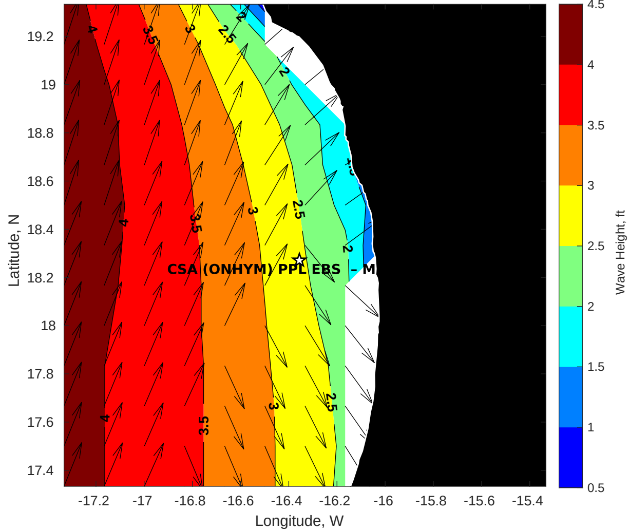
Wave Height (ft) for CSA (ONHYM) PPL EBS - Mauritania at 16-Sep-2025 09:00:00
