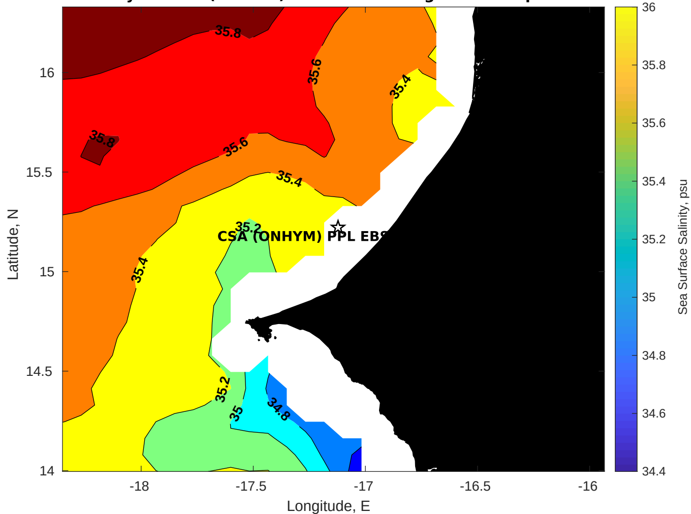
Surface Salinity for CSA (ONHYM) PPL EBS - Senegal at 15-Sep-2025 00:00:00
