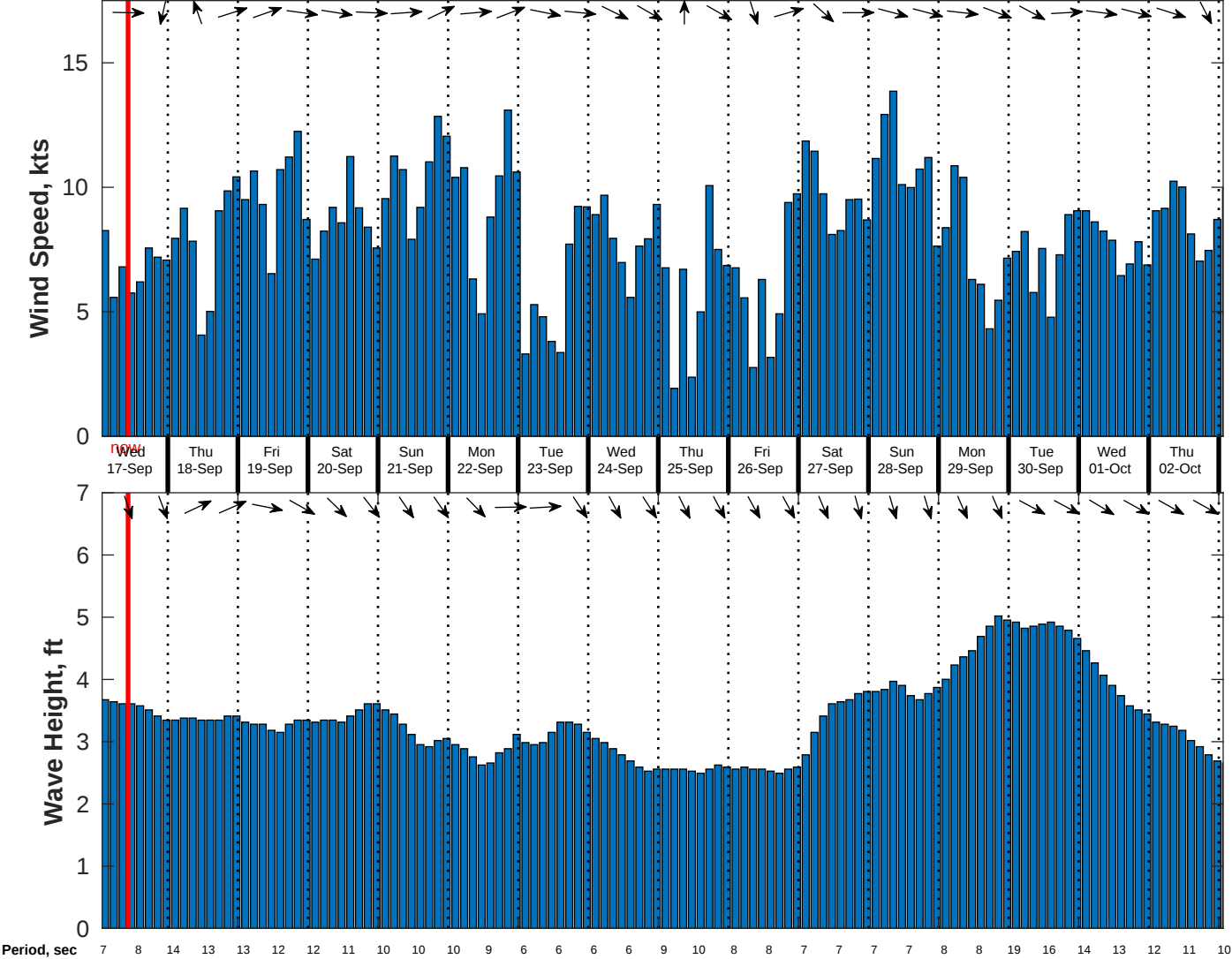
Wind & Wave Forecast for CSA (ONHYM) PPL EBS - Senegal from 16-Sep-2025 01:00:00 to 02-Oct-2025 01:00:00
