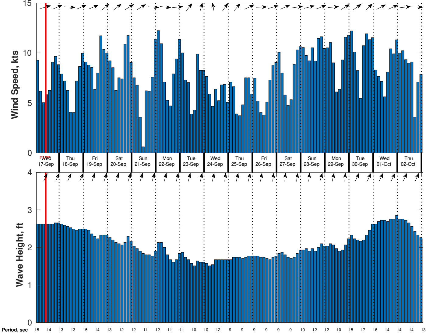
Wind & Wave Forecast for CSA (ONHYM) PPL EBS - Sierra Leone from 16-Sep-2025 01:00:00 to 02-Oct-2025 01:00:00
