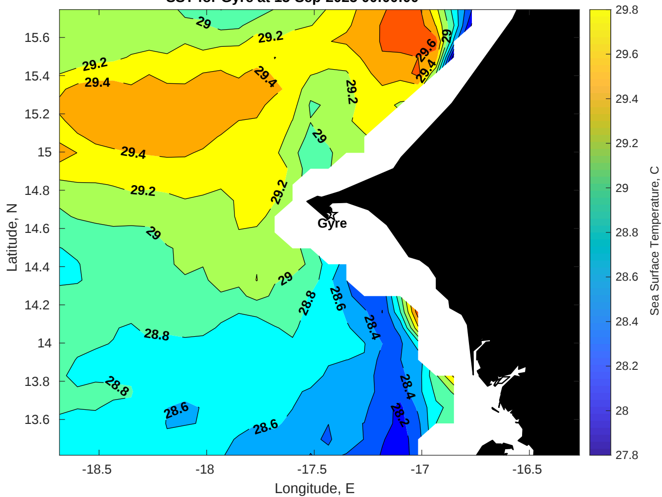
SST for Gyre at 15-Sep-2025 00:00:00
