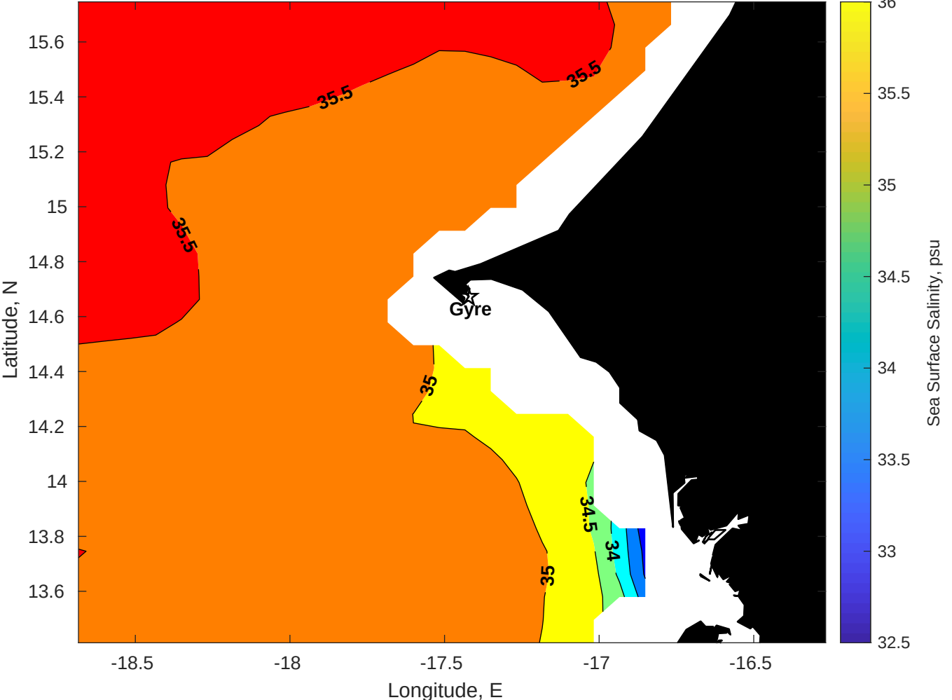
Surface Salinity for Gyre at 15-Sep-2025 00:00:00
