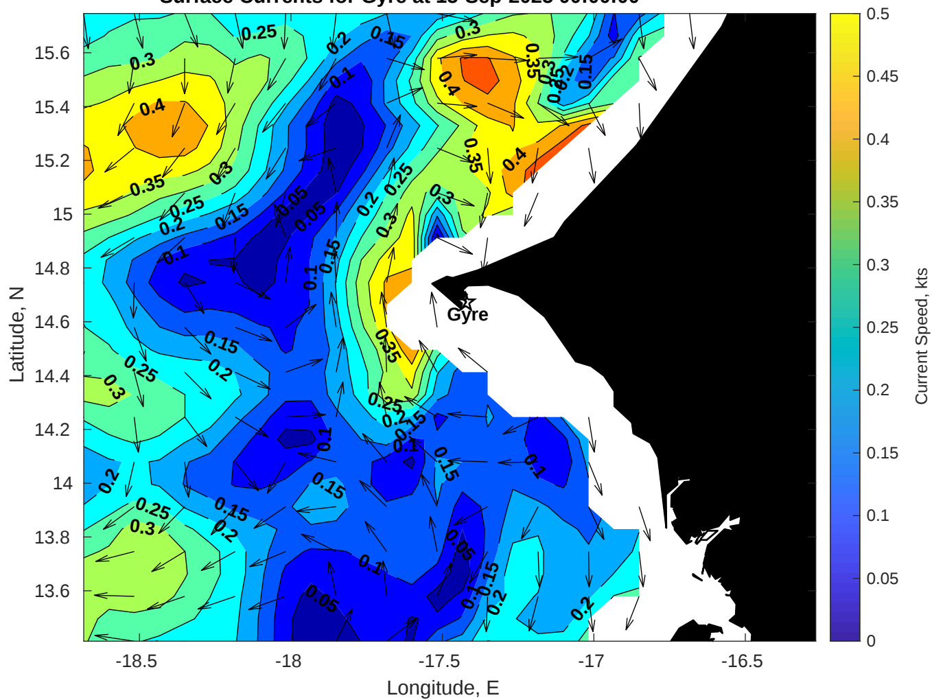
Surface Currents for Gyre at 15-Sep-2025 00:00:00
