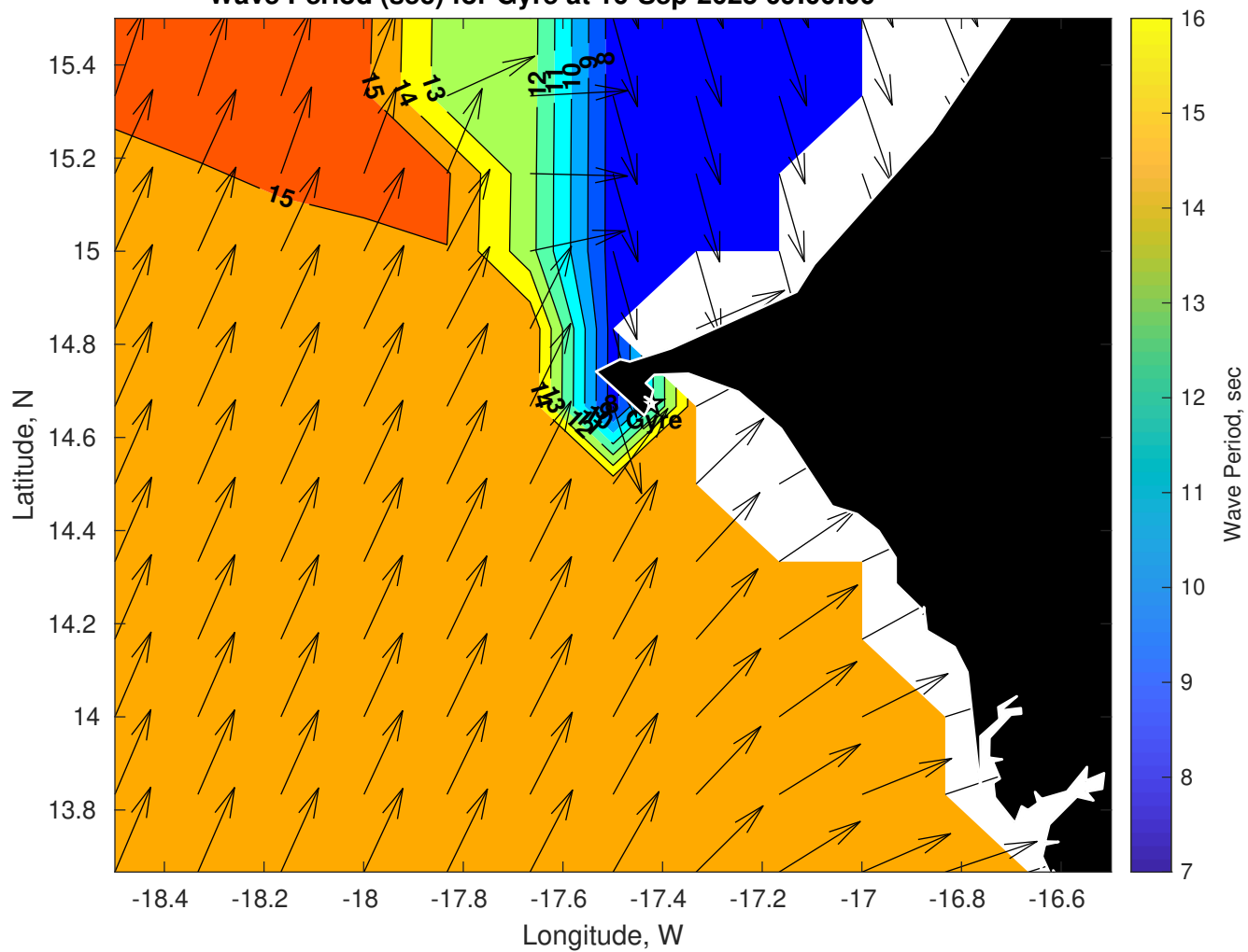
Wave Period (sec) for Gyre at 16-Sep-2025 09:00:00
