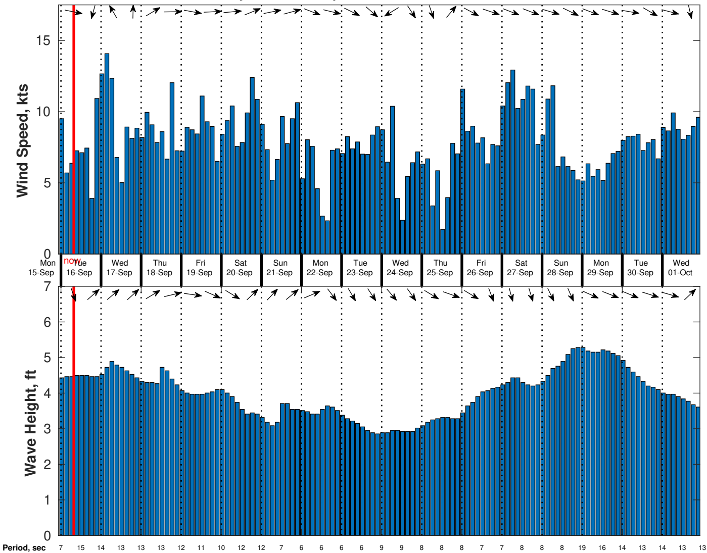
Wind & Wave Forecast for Gyre from 15-Sep-2025 23:00:00 to 01-Oct-2025 23:00:00
