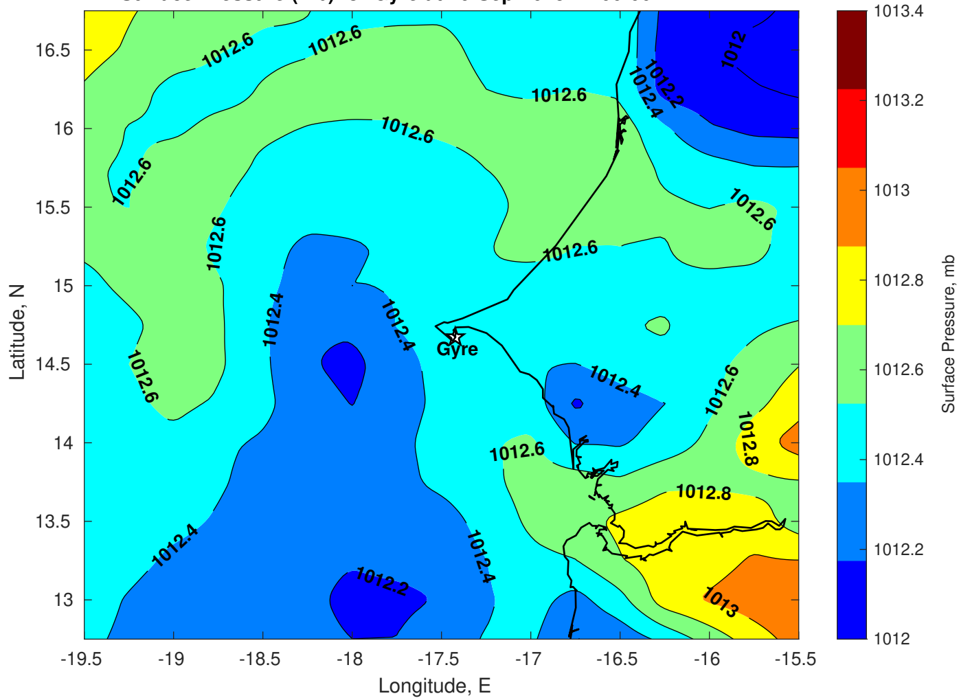
Surface Pressure (mb) for Gyre at 16-Sep-2025 12:00:00
