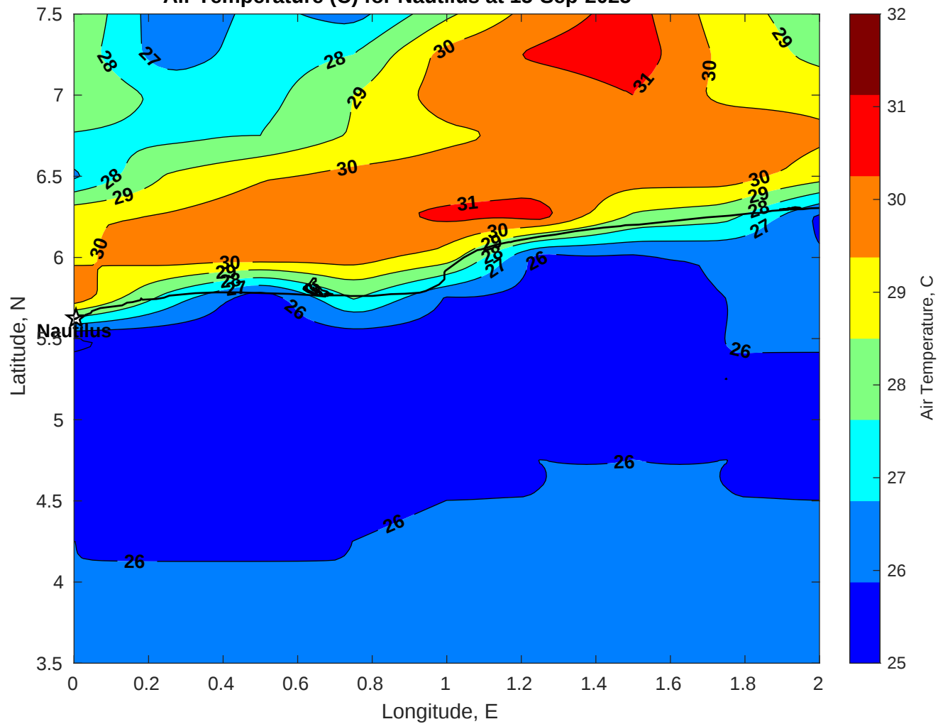
Air Temperature (C) for Nautilus at 15-Sep-2025
