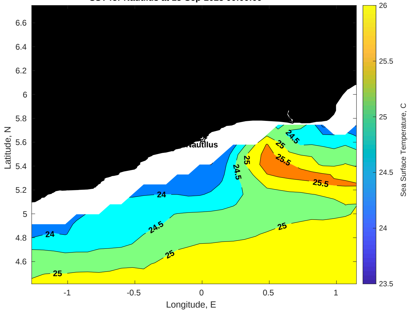
SST for Nautilus at 15-Sep-2025 00:00:00
