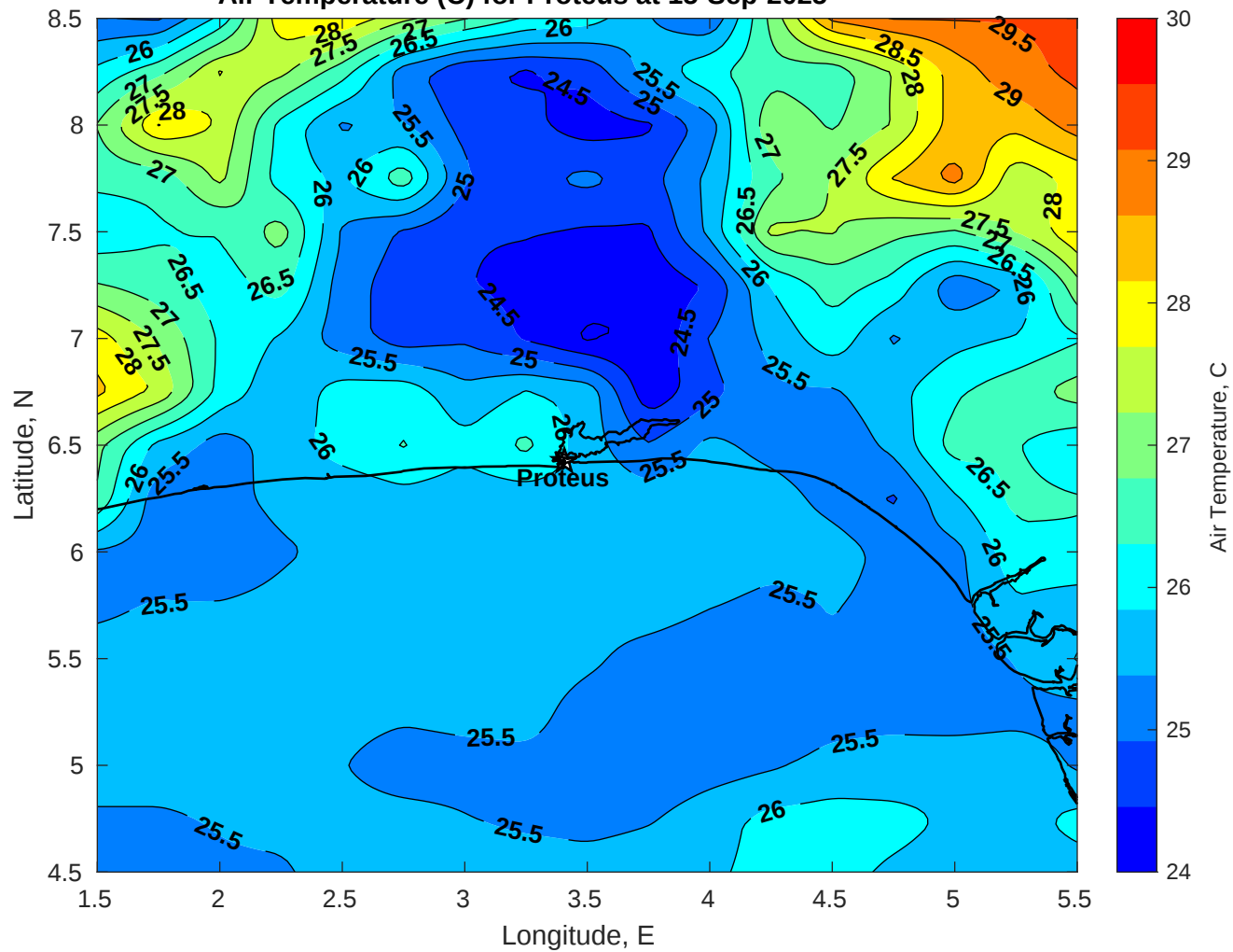
Air Temperature (C) for Proteus at 15-Sep-2025
