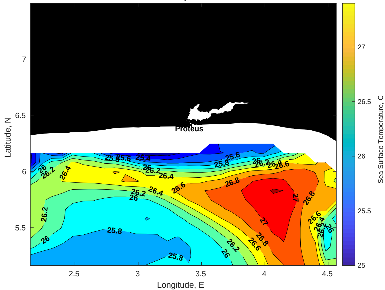
SST for Proteus at 15-Sep-2025 00:00:00
