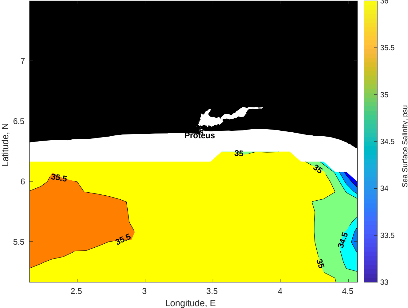
Surface Salinity for Proteus at 15-Sep-2025 00:00:00
