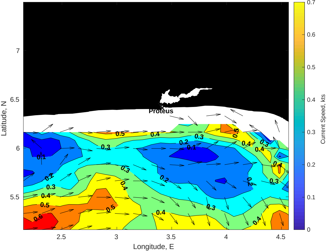
Surface Currents for Proteus at 15-Sep-2025 00:00:00
