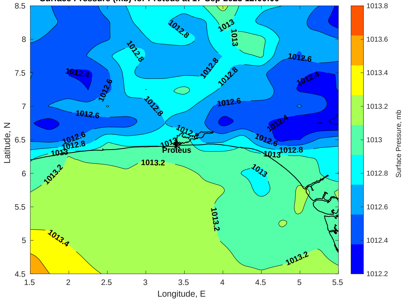
Surface Pressure (mb) for Proteus at 17-Sep-2025 12:00:00
