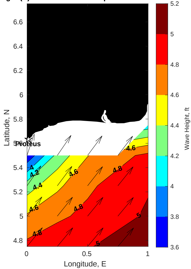
Wave Height (ft) for Proteus at 16-Sep-2025 09:00:00
