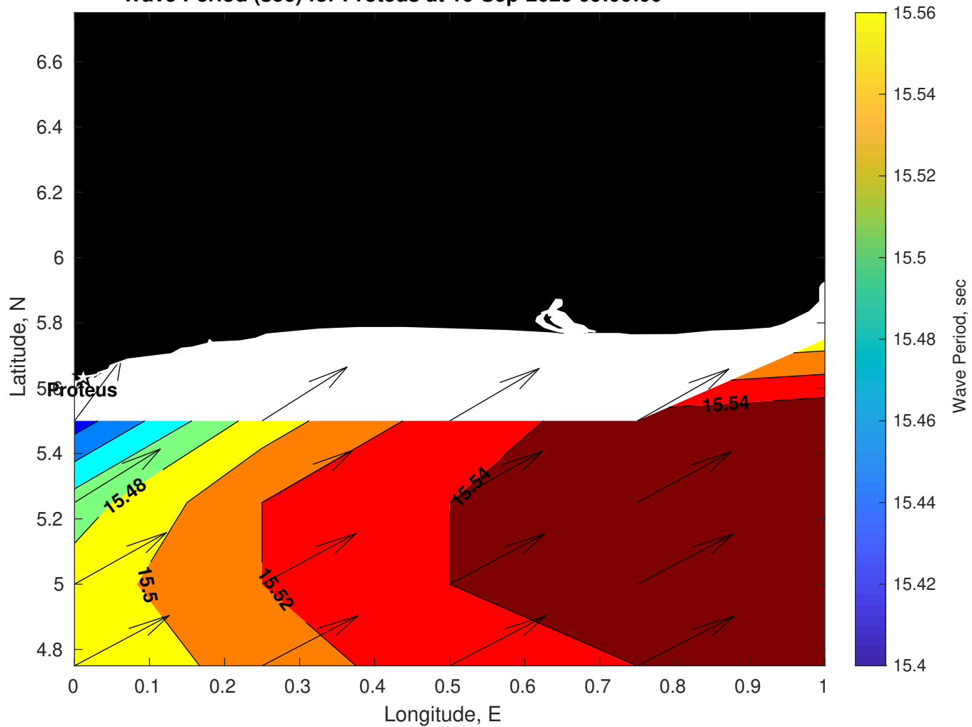
Wave Period (sec) for Proteus at 16-Sep-2025 09:00:00
