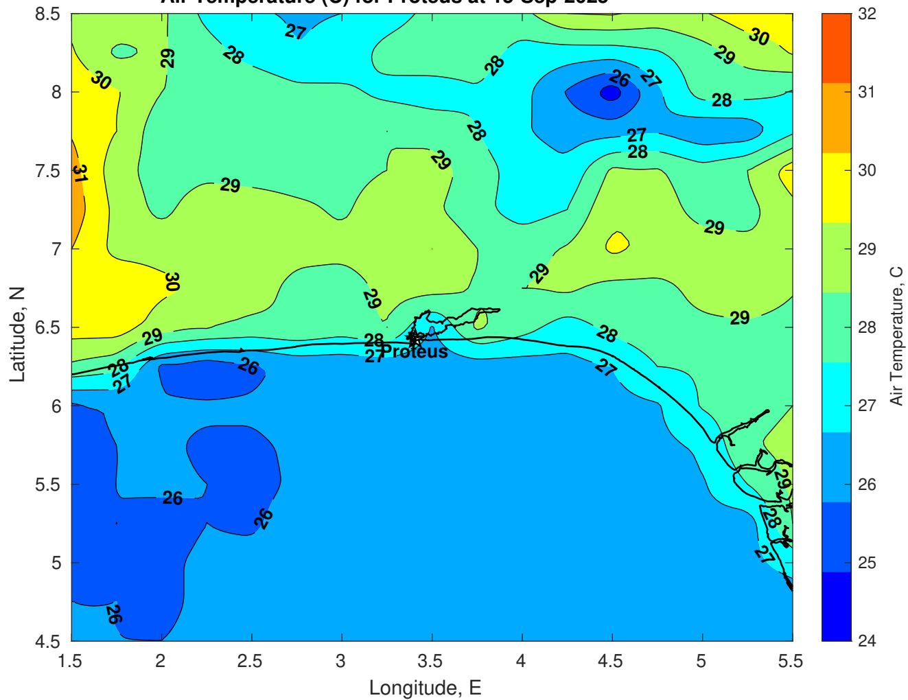
Air Temperature (C) for Proteus at 15-Sep-2025
