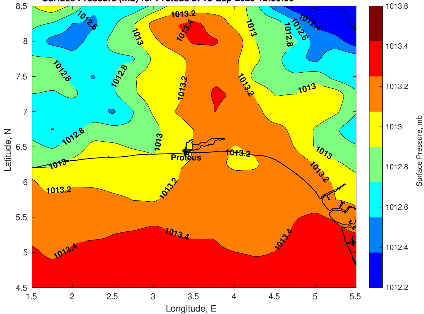
Surface Pressure (mb) for Proteus at 16-Sep-2025 12:00:00
