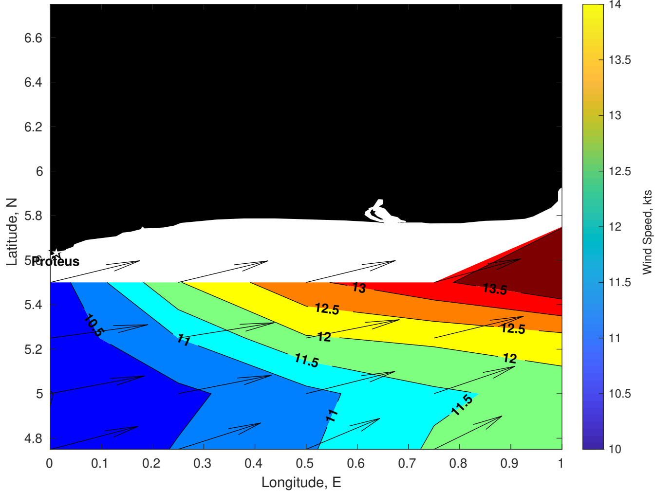
Winds (kts) for Proteus at 16-Sep-2025 09:00:00
