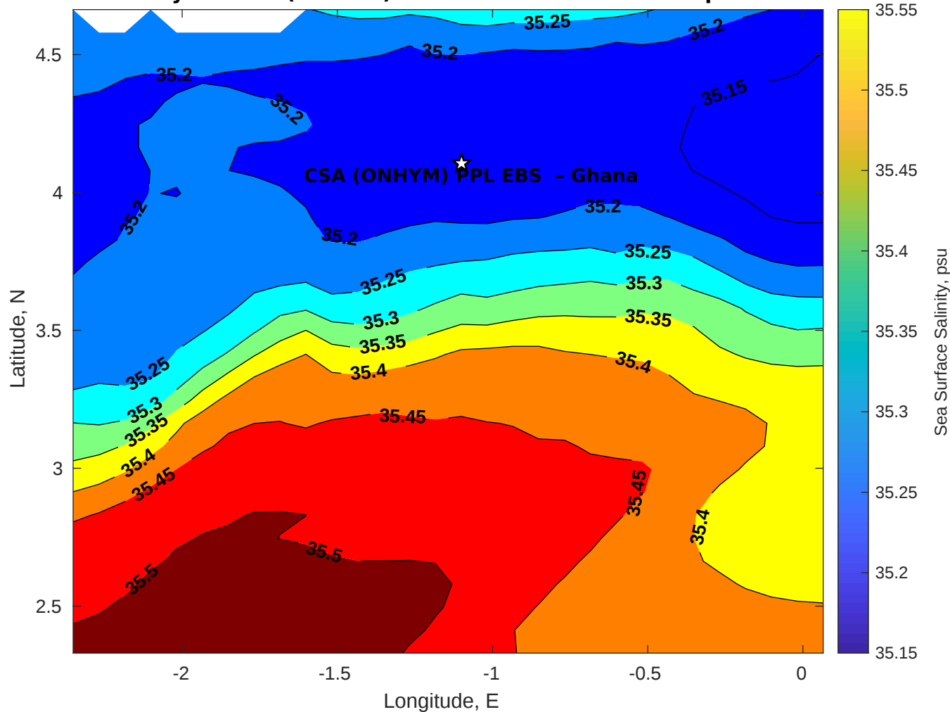
Surface Salinity for CSA (ONHYM) PPL EBS - Ghana at 15-Sep-2025 00:00:00
