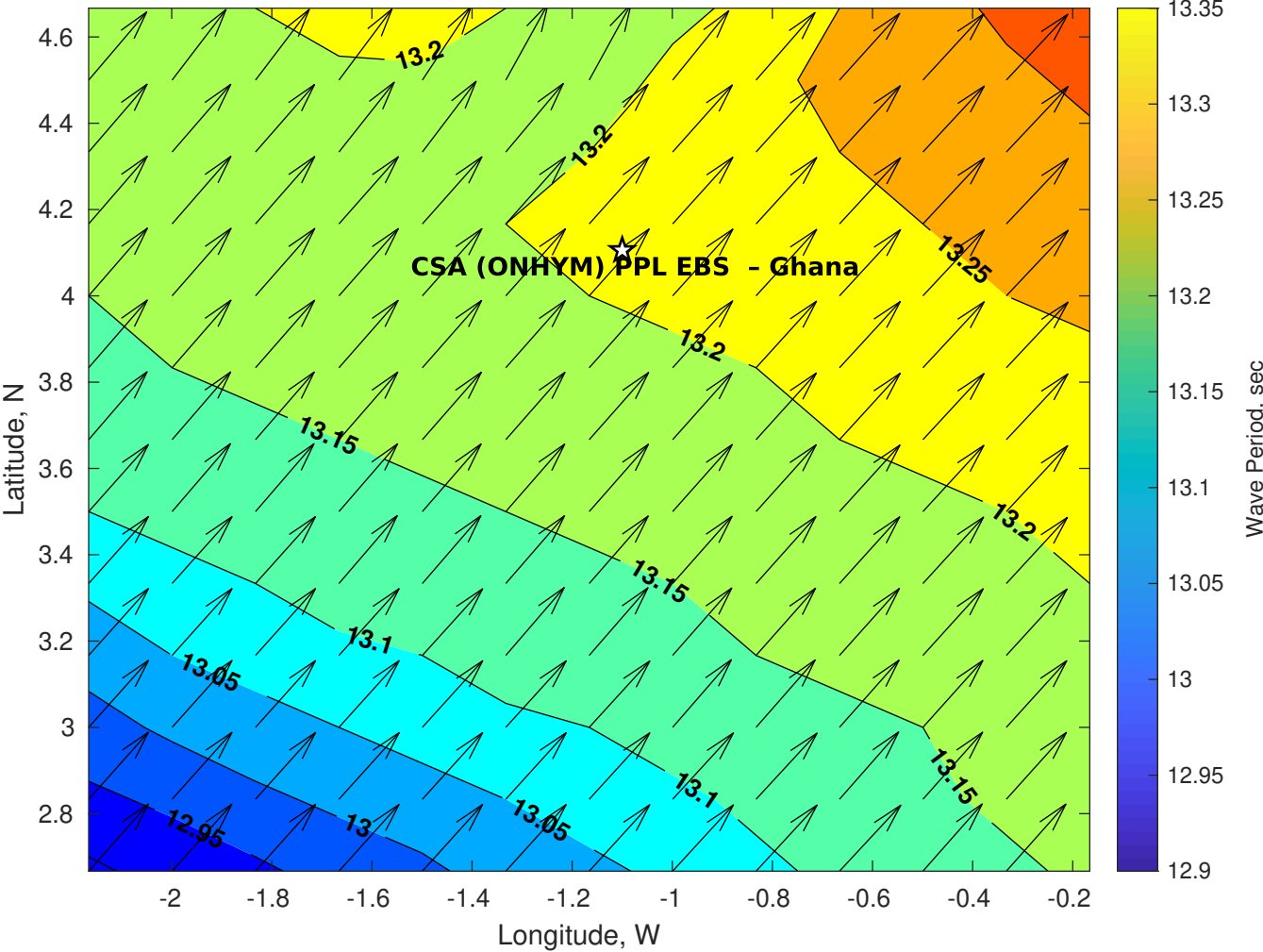
Wave Period (sec) for CSA (ONHYM) PPL EBS - Ghana at 17-Sep-2025 09:00:00
