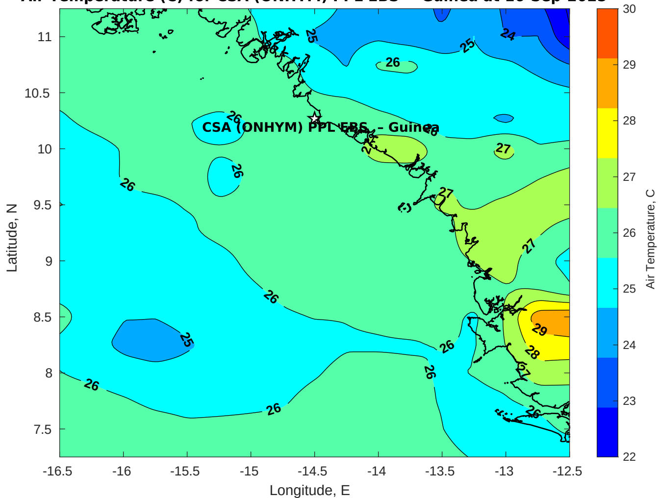
Air Temperature (C) for CSA (ONHYM) PPL EBS - Guinea at 16-Sep-2025
