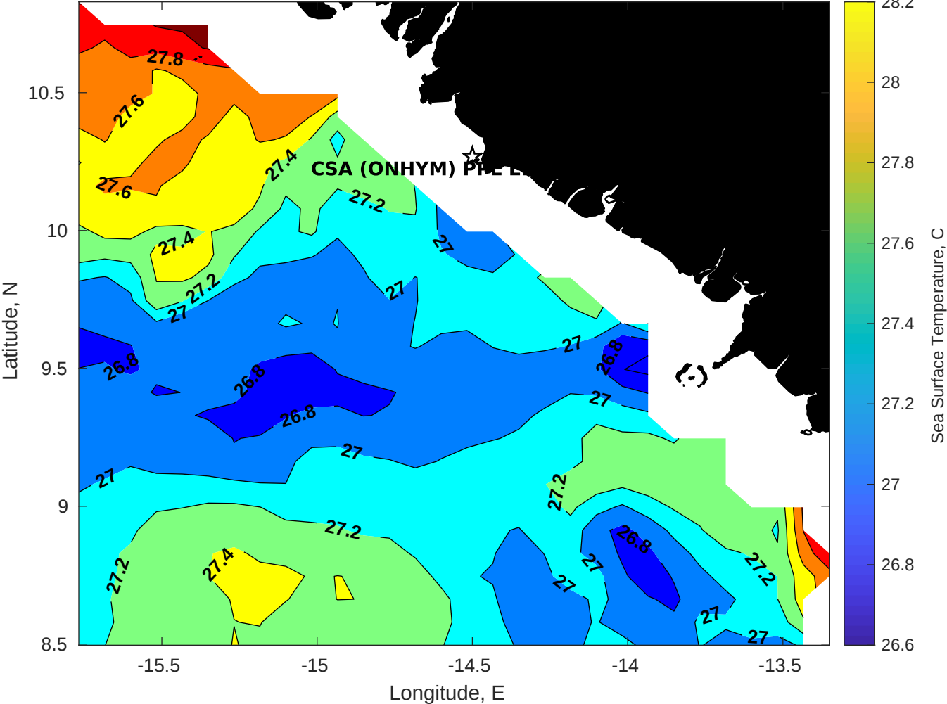
SST for CSA (ONHYM) PPL EBS - Guinea at 16-Sep-2025 00:00:00
