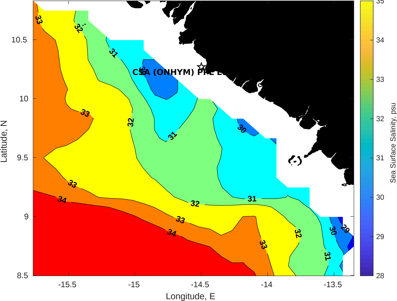
Surface Salinity for CSA (ONHYM) PPL EBS - Guinea at 16-Sep-2025 00:00:00
