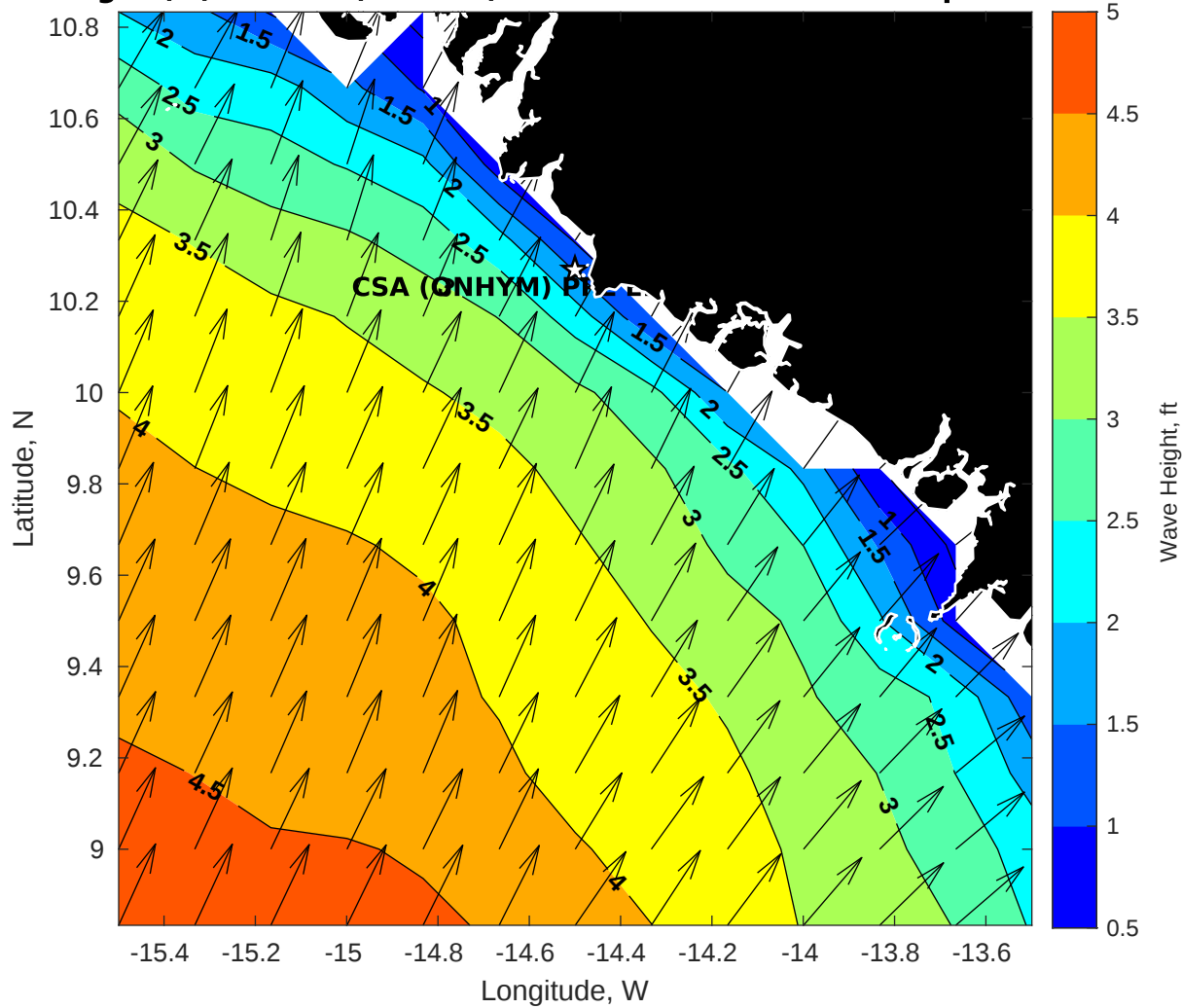
Wave Height (ft) for CSA (ONHYM) PPL EBS - Guinea at 17-Sep-2025 09:00:00
