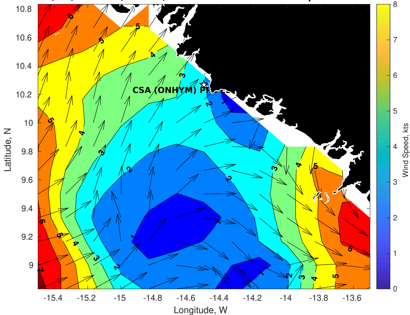
Winds (kts) for CSA (ONHYM) PPL EBS - Guinea at 17-Sep-2025 09:00:00
