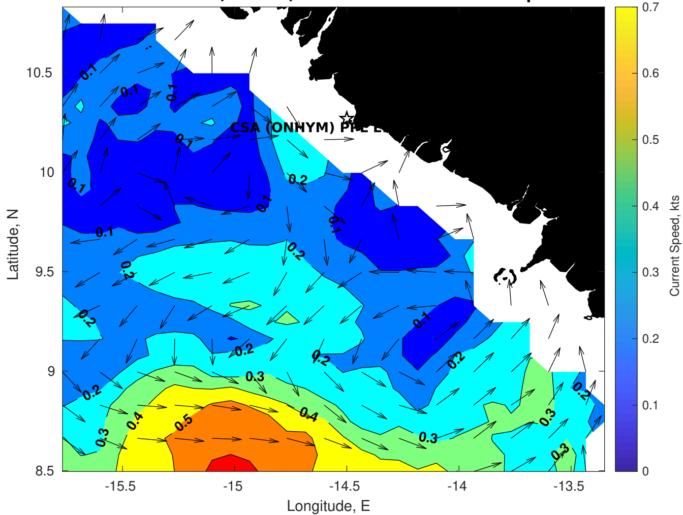
Surface Currents for CSA (ONHYM) PPL EBS - Guinea at 16-Sep-2025 00:00:00
