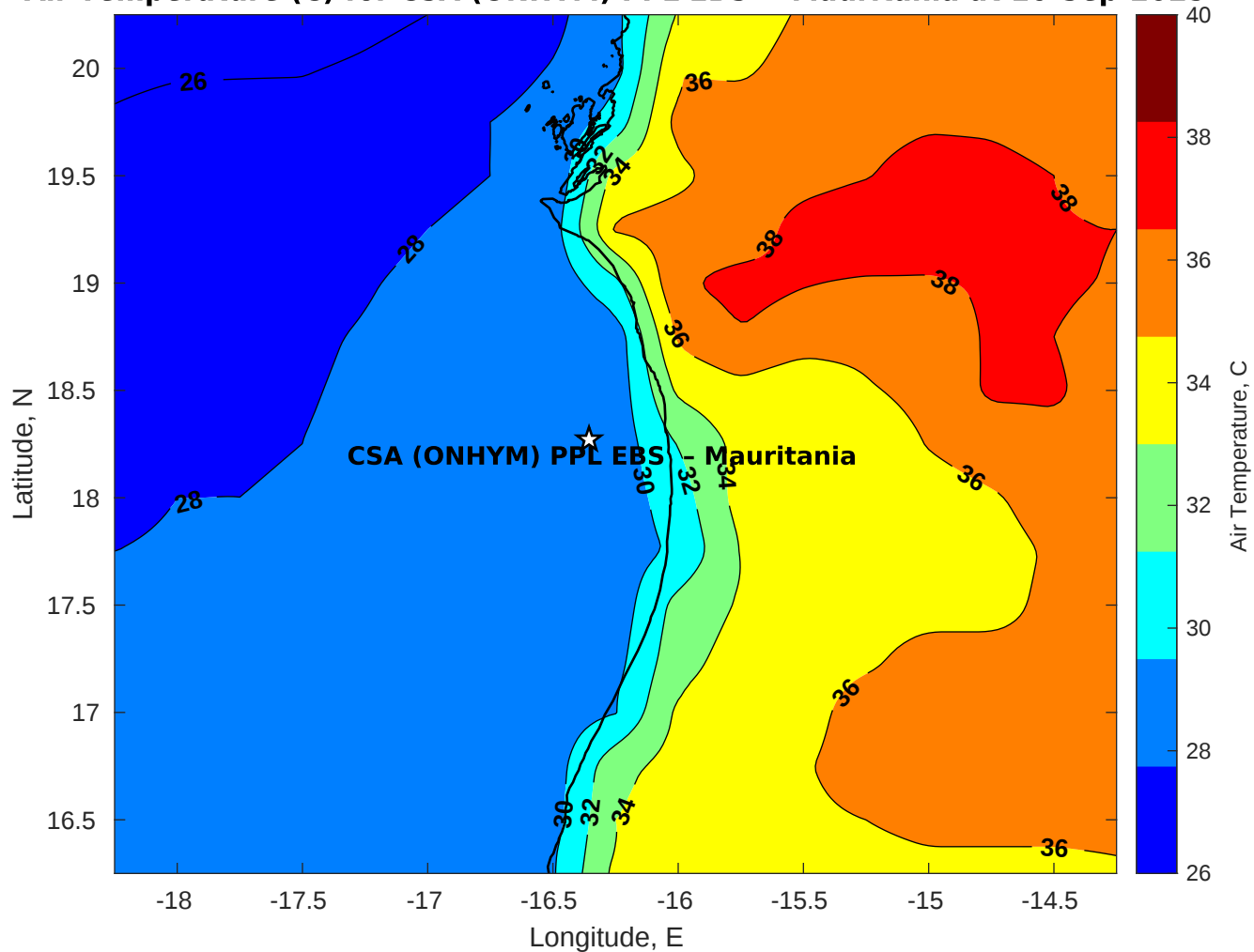
Air Temperature (C) for CSA (ONHYM) PPL EBS - Mauritania at 16-Sep-2025
