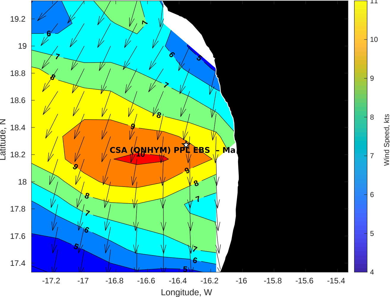
Winds (kts) for CSA (ONHYM) PPL EBS - Mauritania at 17-Sep-2025 09:00:00
