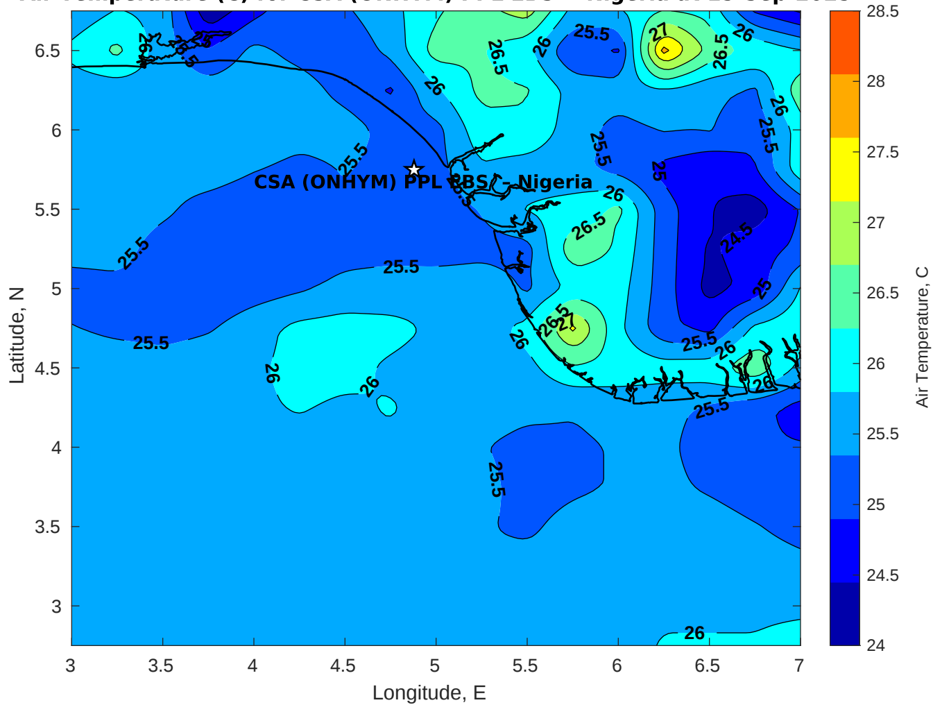
Air Temperature (C) for CSA (ONHYM) PPL EBS - Nigeria at 15-Sep-2025
