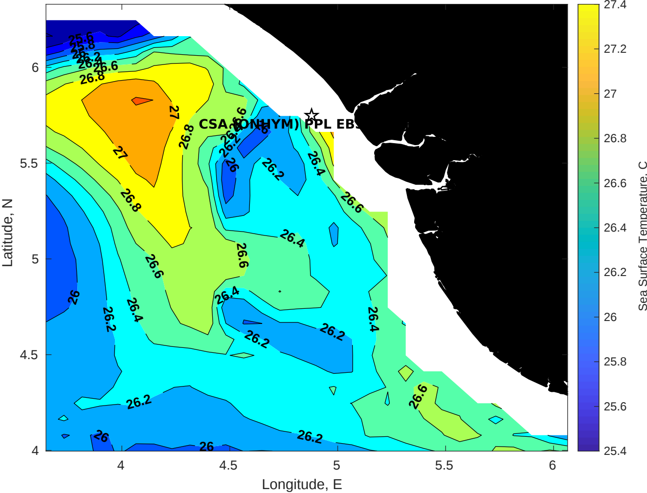
SST for CSA (ONHYM) PPL EBS - Nigeria at 15-Sep-2025 00:00:00
