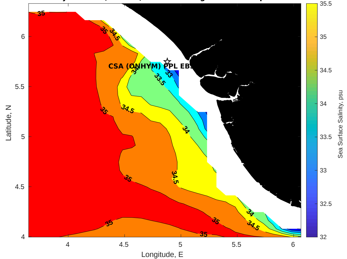
Surface Salinity for CSA (ONHYM) PPL EBS - Nigeria at 15-Sep-2025 00:00:00
