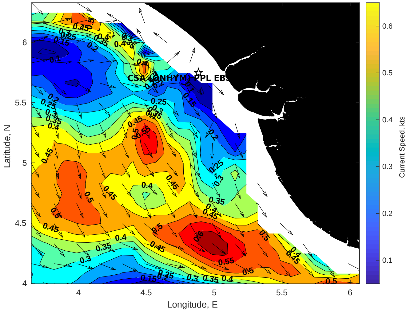
Surface Currents for CSA (ONHYM) PPL EBS - Nigeria at 15-Sep-2025 00:00:00
