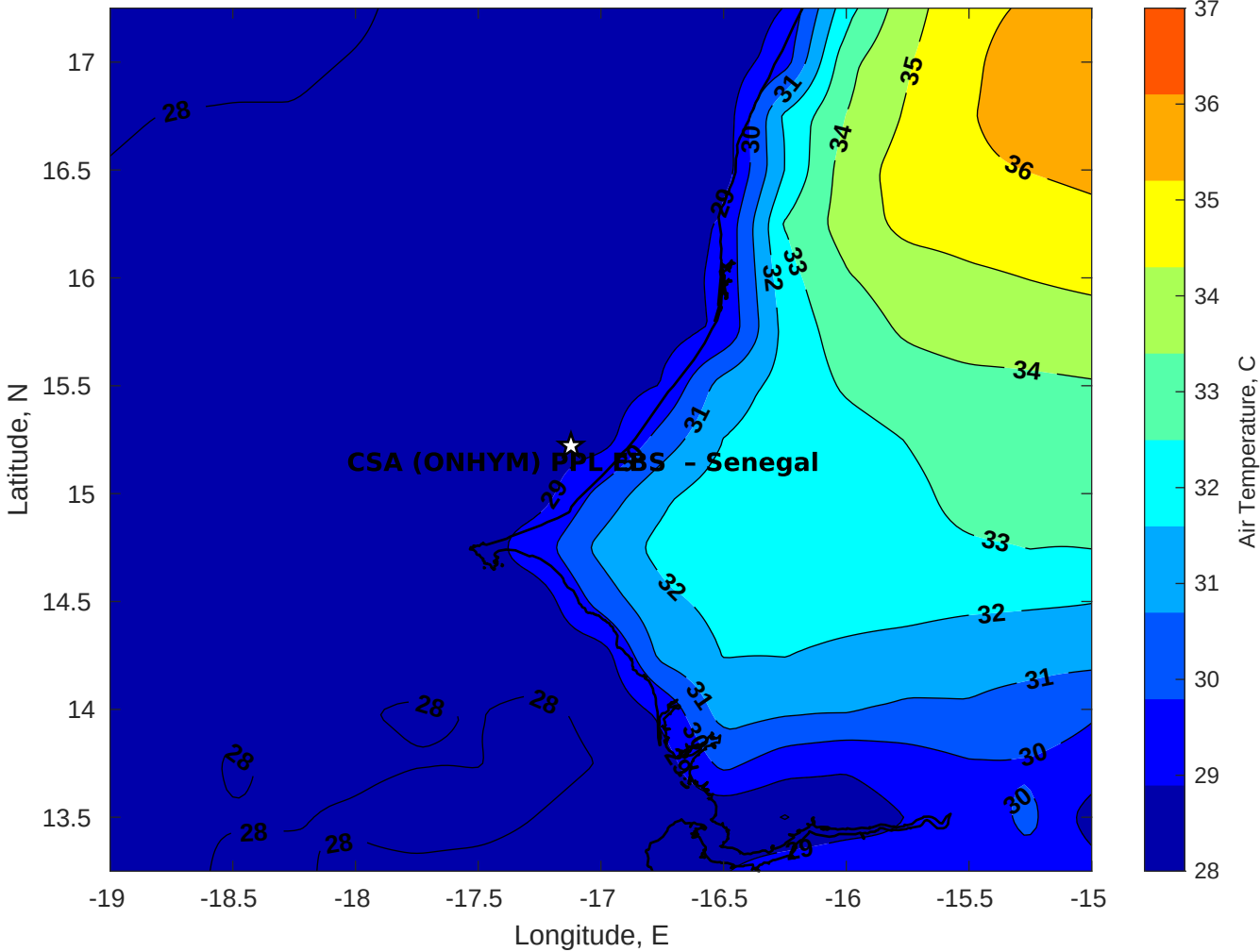
Air Temperature (C) for CSA (ONHYM) PPL EBS - Senegal at 16-Sep-2025
