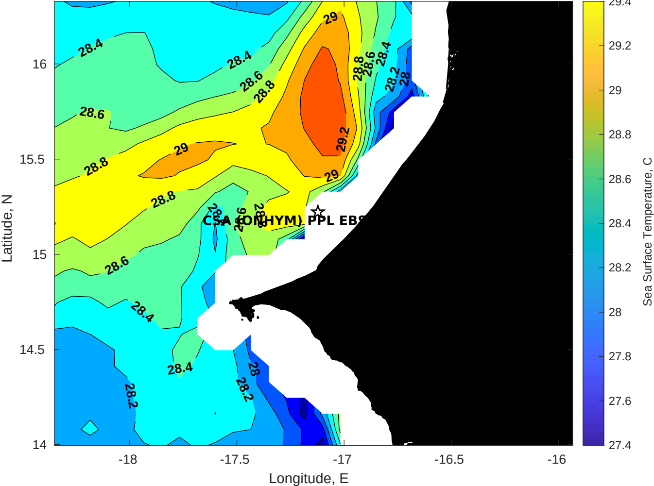
SST for CSA (ONHYM) PPL EBS - Senegal at 16-Sep-2025 00:00:00
