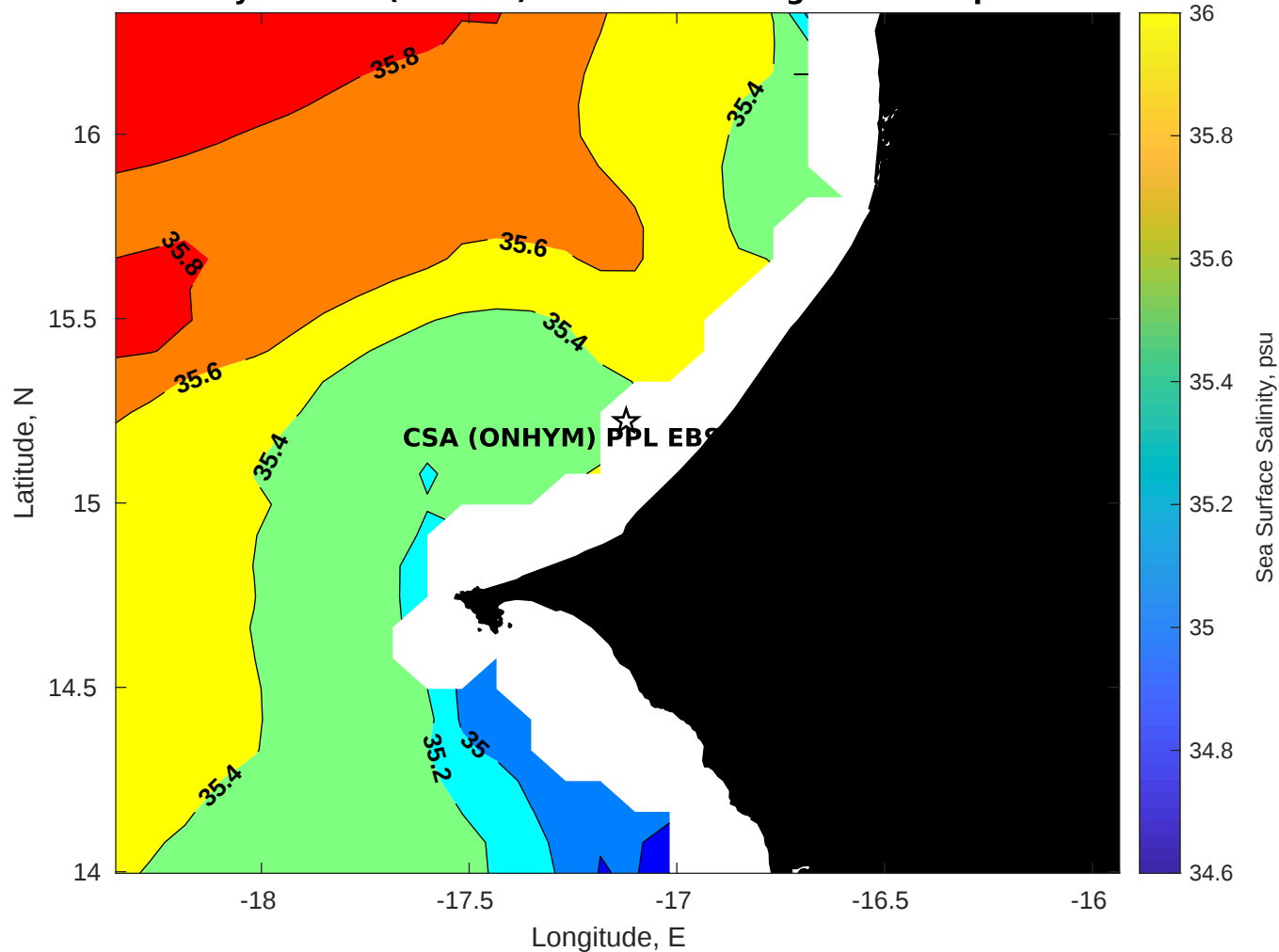
Surface Salinity for CSA (ONHYM) PPL EBS - Senegal at 16-Sep-2025 00:00:00
