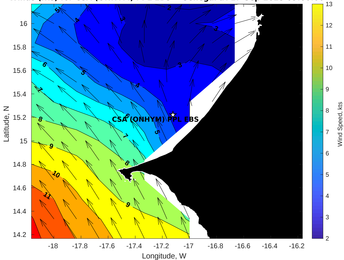
Winds (kts) for CSA (ONHYM) PPL EBS - Senegal at 17-Sep-2025 09:00:00
