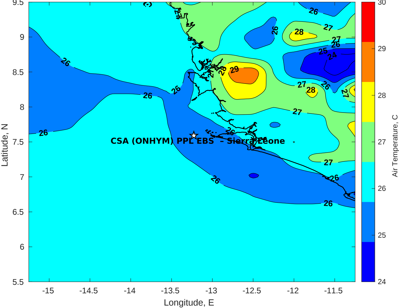
Air Temperature (C) for CSA (ONHYM) PPL EBS - Sierra Leone at 16-Sep-2025
