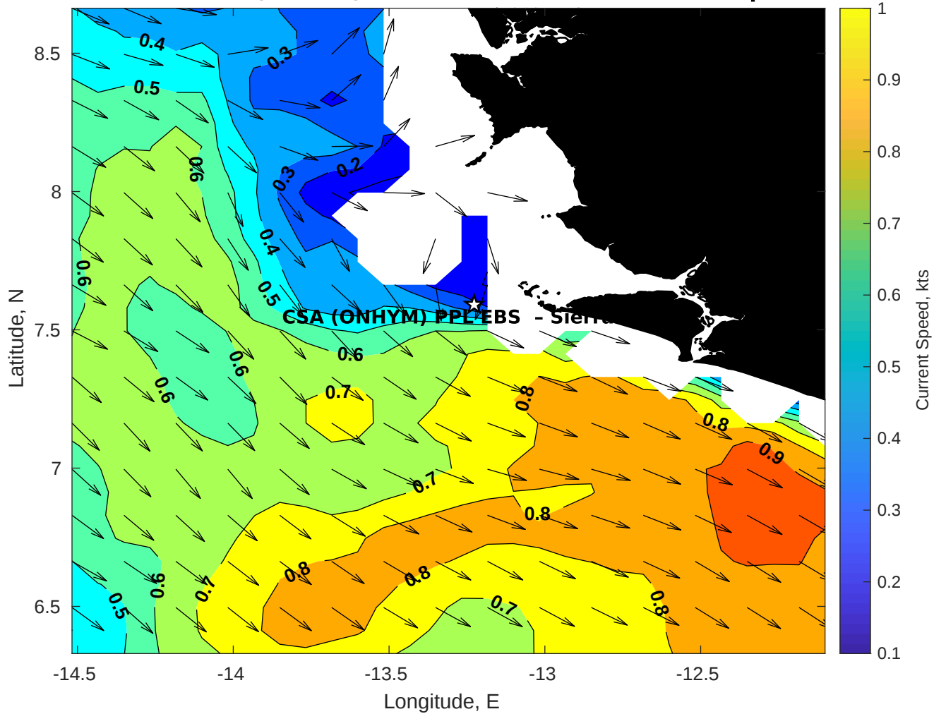
Surface Currents for CSA (ONHYM) PPL EBS - Sierra Leone at 16-Sep-2025 00:00:00
