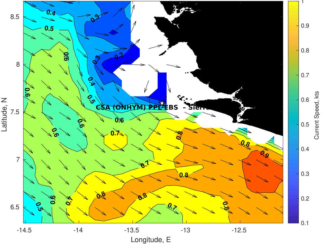
Surface Currents for CSA (ONHYM) PPL EBS - Sierra Leone at 16-Sep-2025 00:00:00
