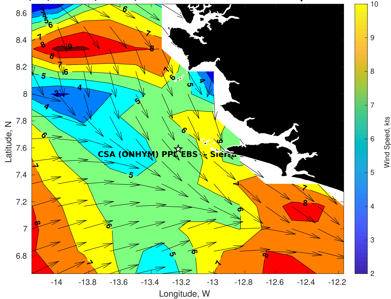
Winds (kts) for CSA (ONHYM) PPL EBS - Sierra Leone at 17-Sep-2025 09:00:00
