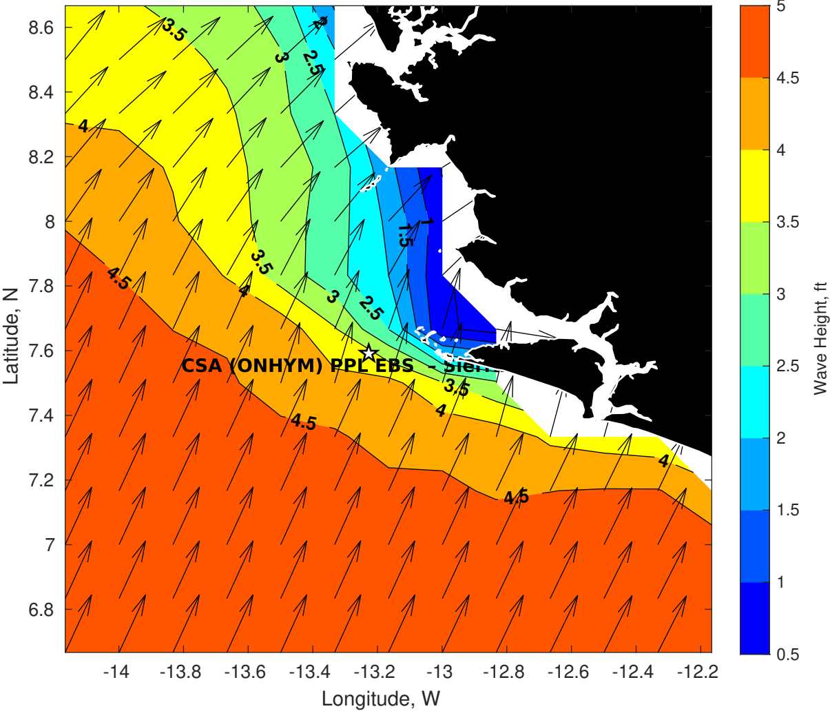
Wave Height (ft) for CSA (ONHYM) PPL EBS - Sierra Leone at 17-Sep-2025 09:00:00
