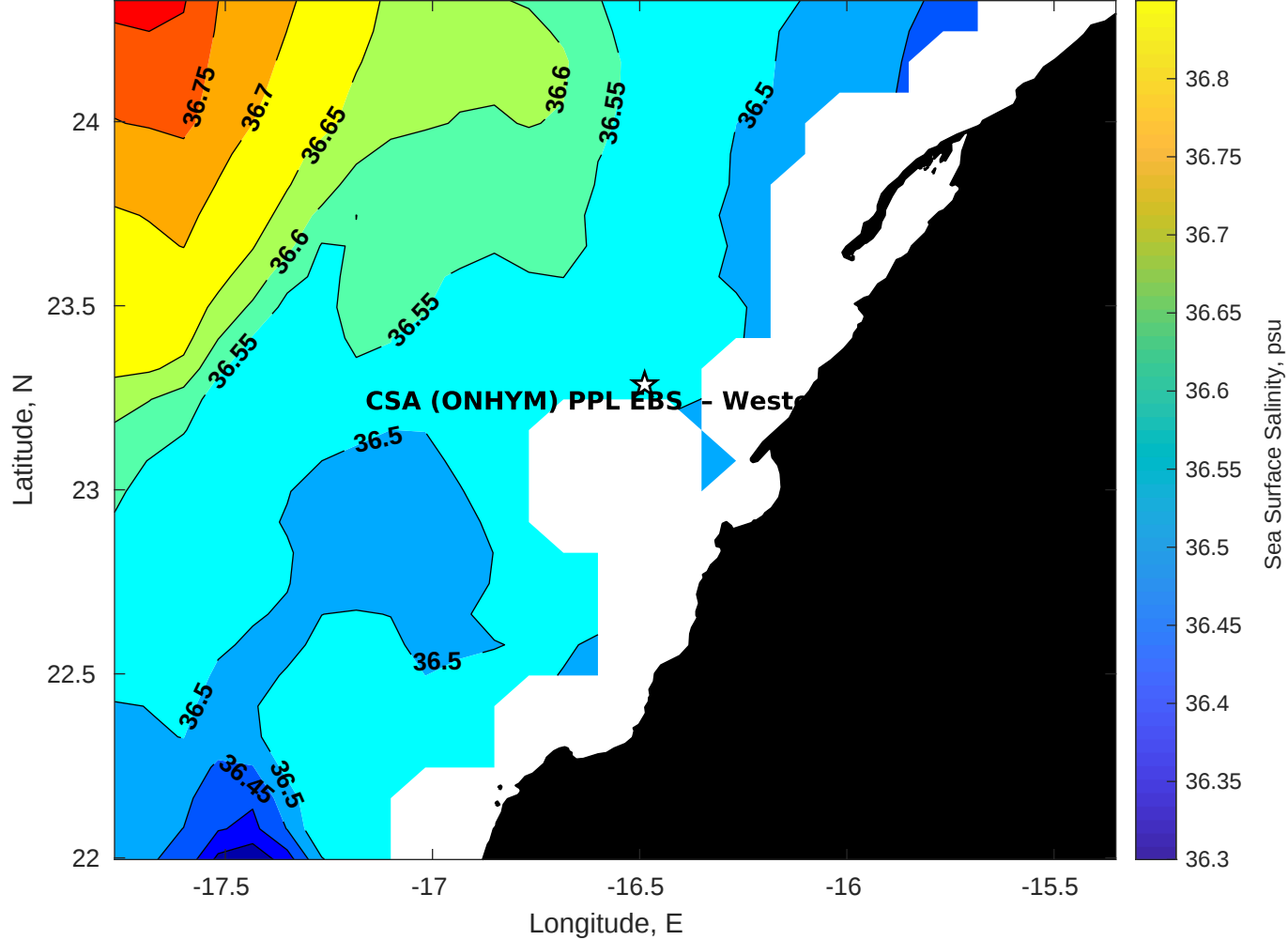
Surface Salinity for CSA (ONHYM) PPL EBS - Western Sahara at 16-Sep-2025 00:00:00
