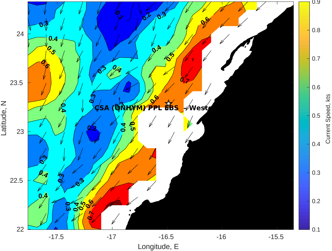
Surface Currents for CSA (ONHYM) PPL EBS - Western Sahara at 16-Sep-2025 00:00:00
